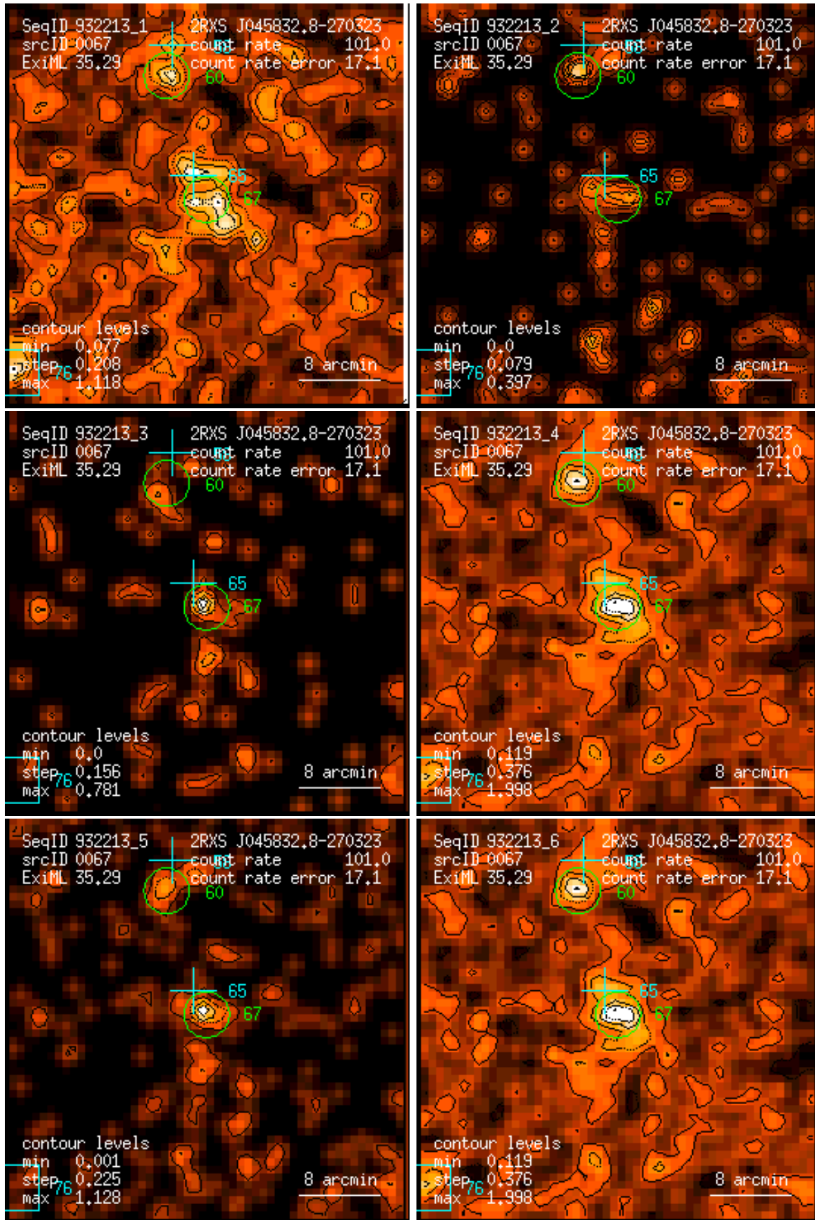
Figure 67: RASS 932213: detection 0067: band rate images, Gaussian filter: (1) PSPC channels 11 – 41, (2) 52 – 90, (3) 91 – 201, (4) 11 – 235, (5) 52 – 201, (6) 11 – 201. Broad band rates in counts/ks. Band rate contour levels in counts/ks/arcmin 2 .
