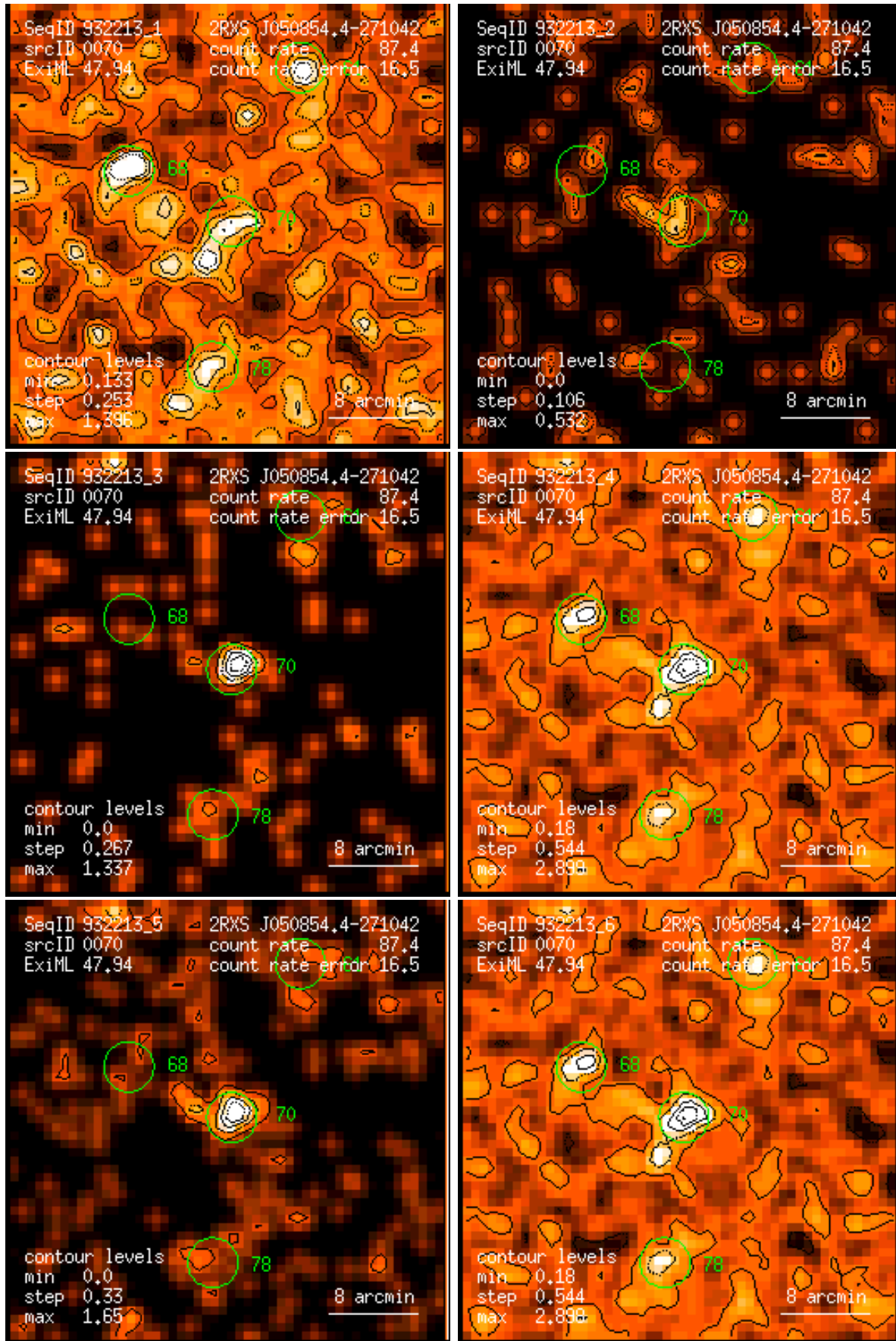
Figure 70: RASS 932213: detection 0070: band rate images, Gaussian filter: (1) PSPC channels 11 – 41, (2) 52 – 90, (3) 91 – 201, (4) 11 – 235, (5) 52 – 201, (6) 11 – 201. Broad band rates in counts/ks. Band rate contour levels in counts/ks/arcmin 2 .
