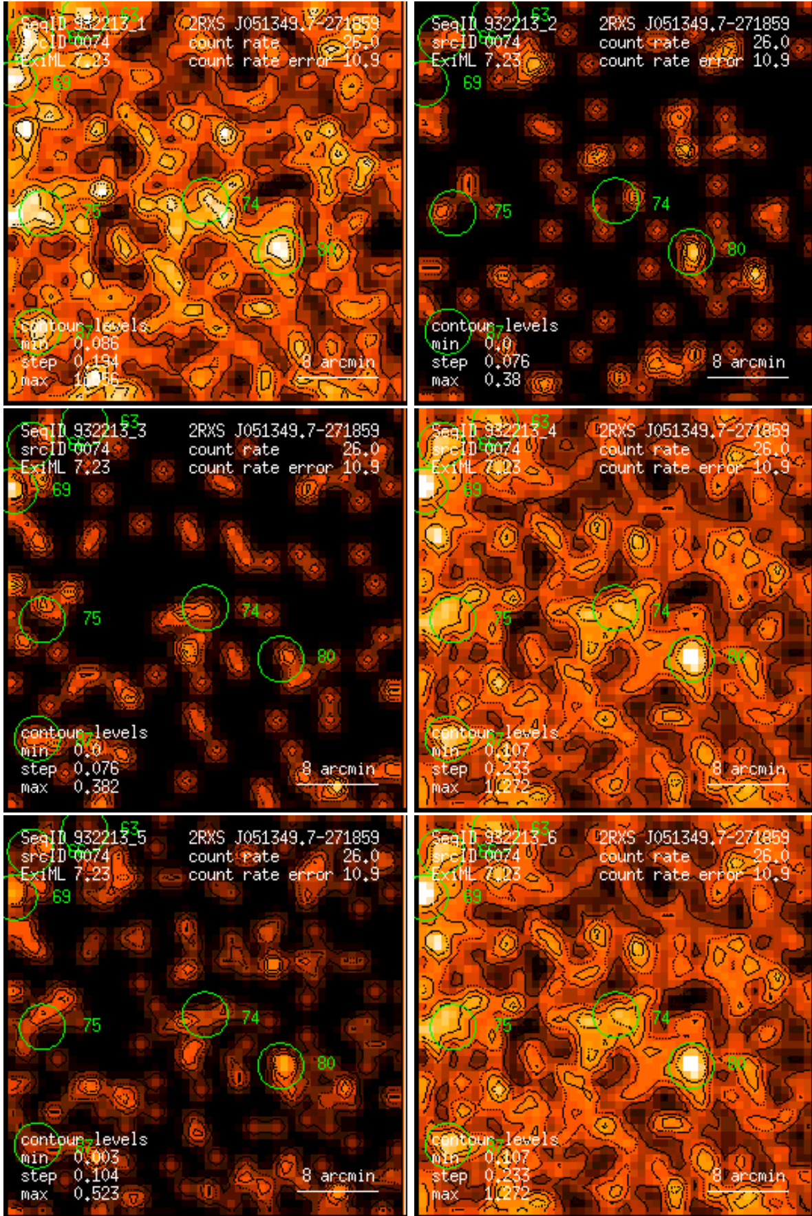
Figure 74: RASS 932213: detection 0074: band rate images, Gaussian filter: (1) PSPC channels 11 – 41, (2) 52 – 90, (3) 91 – 201, (4) 11 – 235, (5) 52 – 201, (6) 11 – 201. Broad band rates in counts/ks. Band rate contour levels in counts/ks/arcmin 2 .
