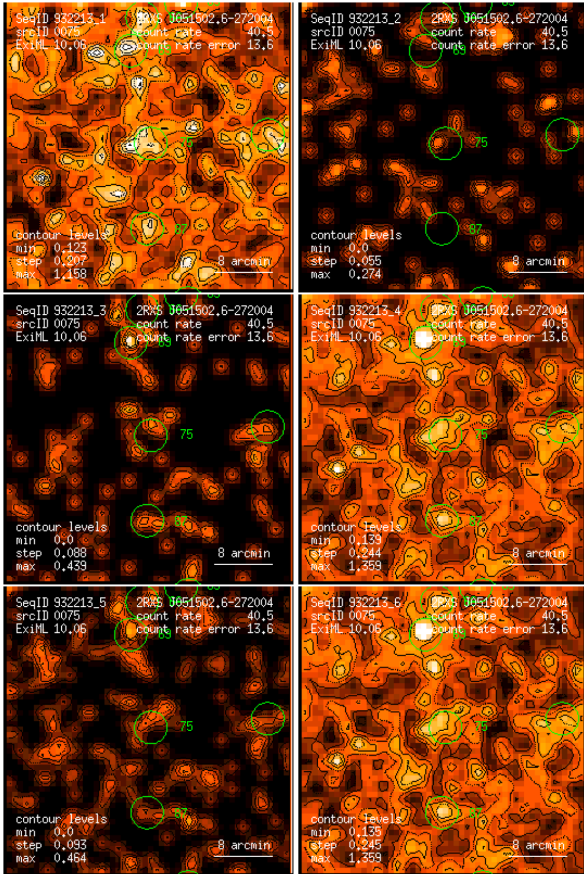
Figure 75: RASS 932213: detection 0075: band rate images, Gaussian filter: (1) PSPC channels 11 – 41, (2) 52 – 90, (3) 91 – 201, (4) 11 – 235, (5) 52 – 201, (6) 11 – 201. Broad band rates in counts/ks. Band rate contour levels in counts/ks/arcmin 2 .
