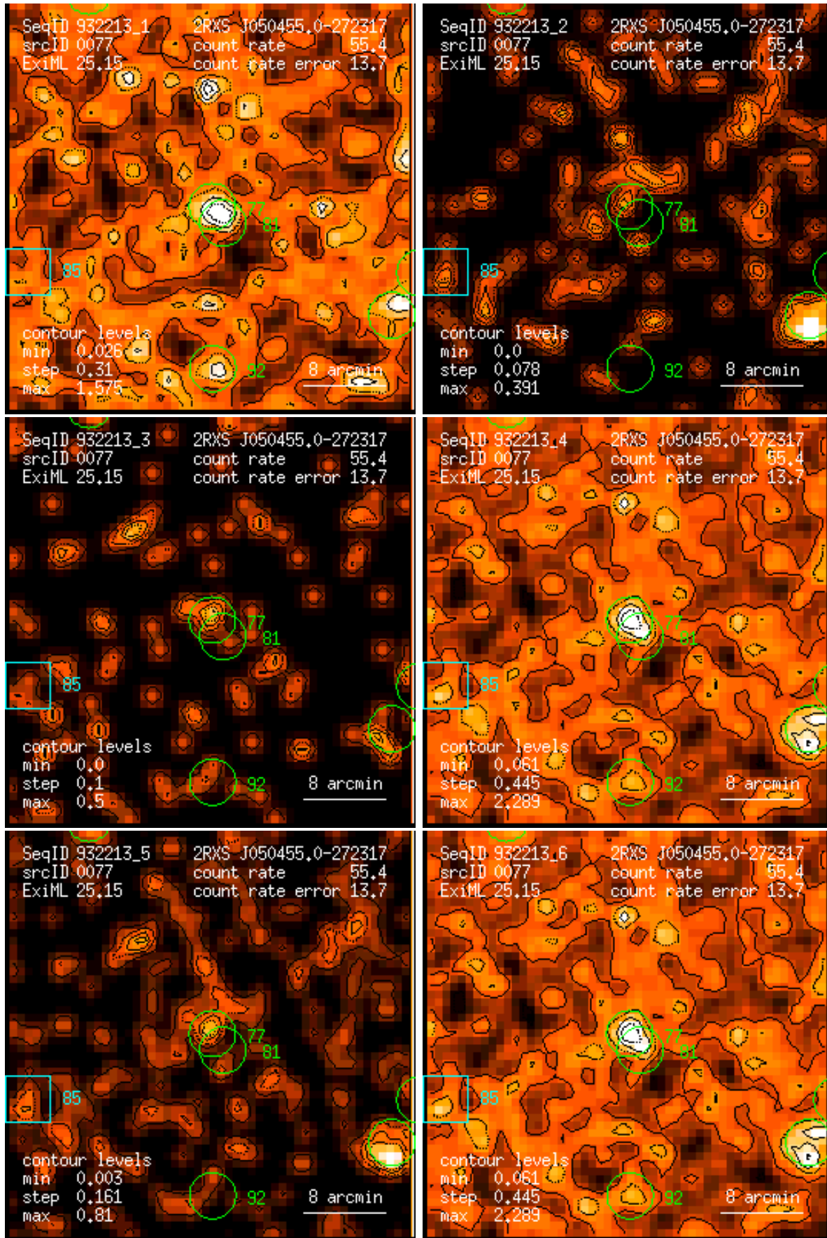
Figure 77: RASS 932213: detection 0077: band rate images, Gaussian filter: (1) PSPC channels 11 – 41, (2) 52 – 90, (3) 91 – 201, (4) 11 – 235, (5) 52 – 201, (6) 11 – 201. Broad band rates in counts/ks. Band rate contour levels in counts/ks/arcmin 2 .
