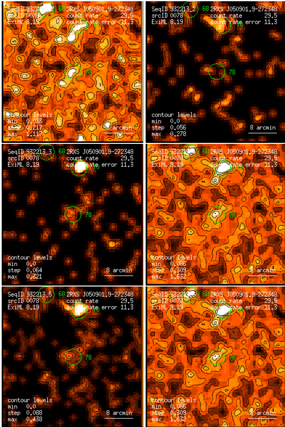
Figure 78: RASS 932213: detection 0078: band rate images, Gaussian filter: (1) PSPC channels 11 – 41, (2) 52 – 90, (3) 91 – 201, (4) 11 – 235, (5) 52 – 201, (6) 11 – 201. Broad band rates in counts/ks. Band rate contour levels in counts/ks/arcmin 2 .
