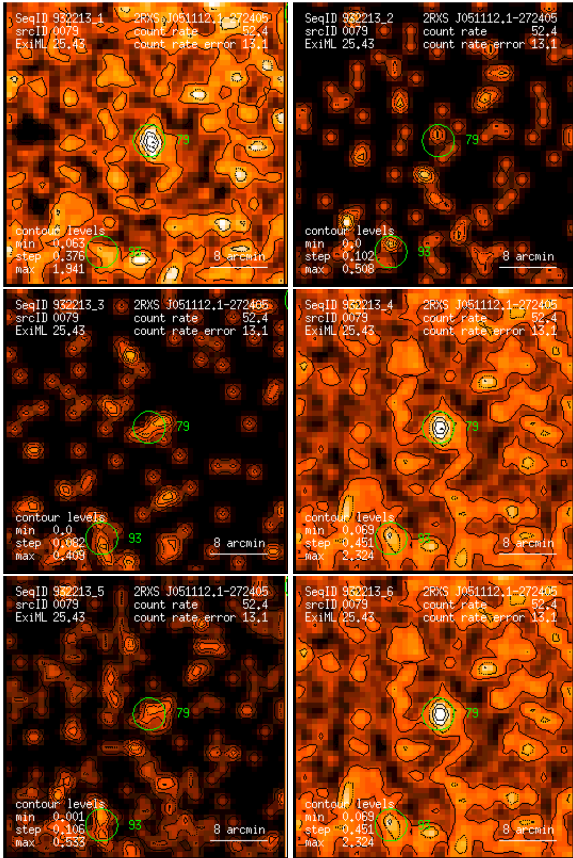
Figure 79: RASS 932213: detection 0079: band rate images, Gaussian filter: (1) PSPC channels 11 – 41, (2) 52 – 90, (3) 91 – 201, (4) 11 – 235, (5) 52 – 201, (6) 11 – 201. Broad band rates in counts/ks. Band rate contour levels in counts/ks/arcmin 2 .
