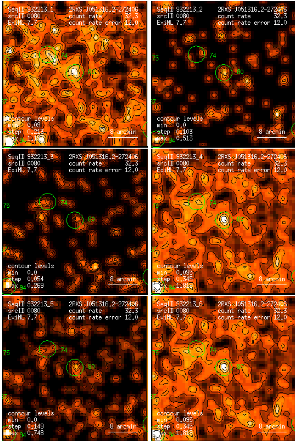
Figure 80: RASS 932213: detection 0080: band rate images, Gaussian filter: (1) PSPC channels 11 – 41, (2) 52 – 90, (3) 91 – 201, (4) 11 – 235, (5) 52 – 201, (6) 11 – 201. Broad band rates in counts/ks. Band rate contour levels in counts/ks/arcmin 2 .
