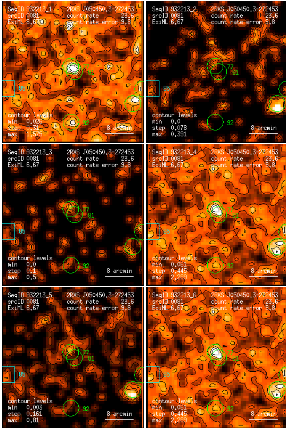
Figure 81: RASS 932213: detection 0081: band rate images, Gaussian filter: (1) PSPC channels 11 – 41, (2) 52 – 90, (3) 91 – 201, (4) 11 – 235, (5) 52 – 201, (6) 11 – 201. Broad band rates in counts/ks. Band rate contour levels in counts/ks/arcmin 2 .
