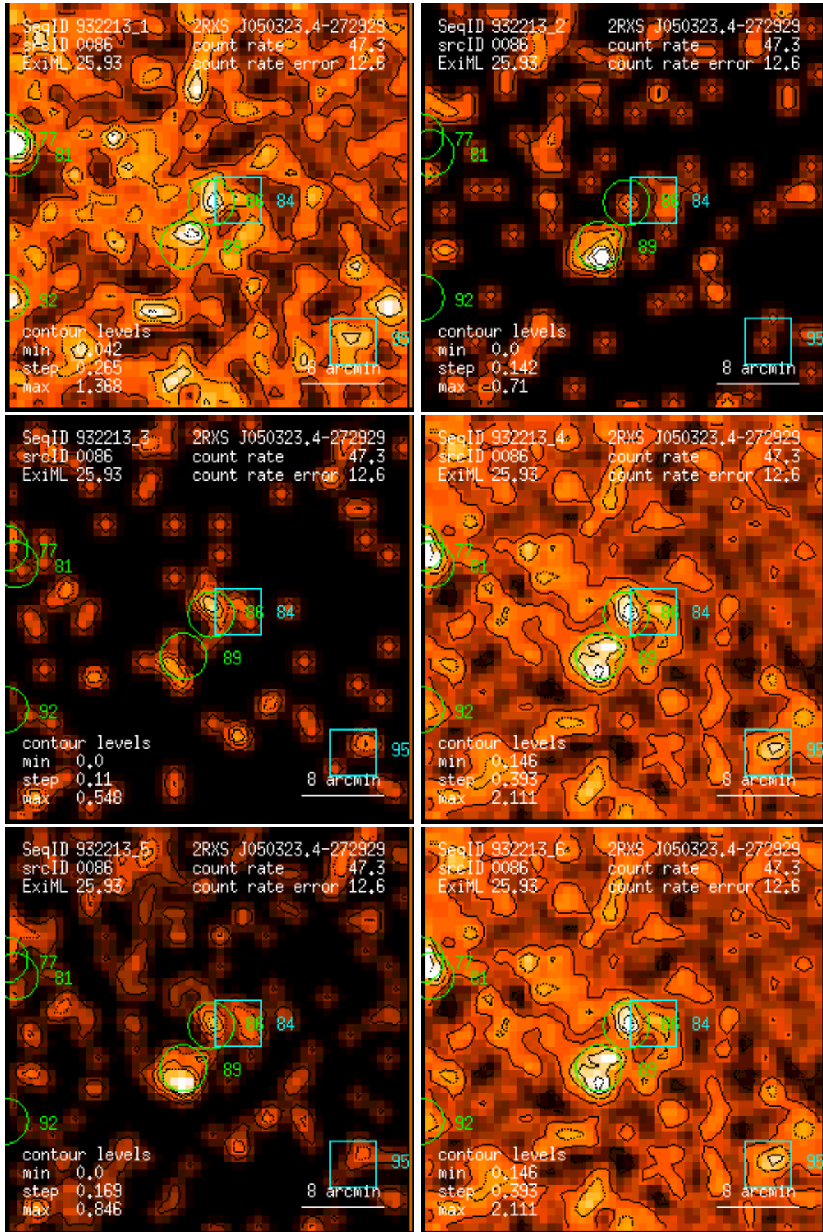
Figure 86: RASS 932213: detection 0086: band rate images, Gaussian filter: (1) PSPC channels 11 – 41, (2) 52 – 90, (3) 91 – 201, (4) 11 – 235, (5) 52 – 201, (6) 11 – 201. Broad band rates in counts/ks. Band rate contour levels in counts/ks/arcmin 2 .
