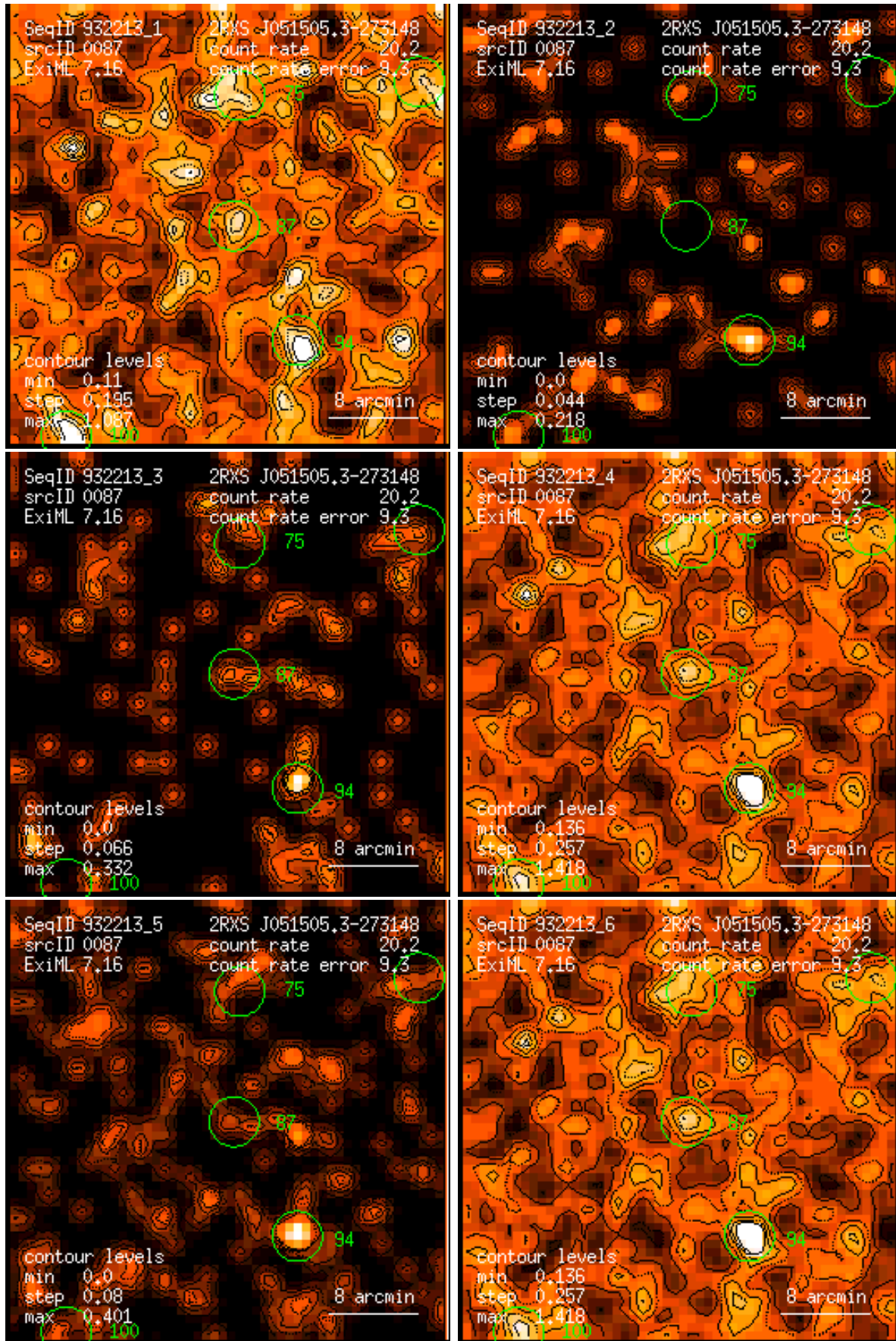
Figure 87: RASS 932213: detection 0087: band rate images, Gaussian filter: (1) PSPC channels 11 – 41, (2) 52 – 90, (3) 91 – 201, (4) 11 – 235, (5) 52 – 201, (6) 11 – 201. Broad band rates in counts/ks. Band rate contour levels in counts/ks/arcmin 2 .
