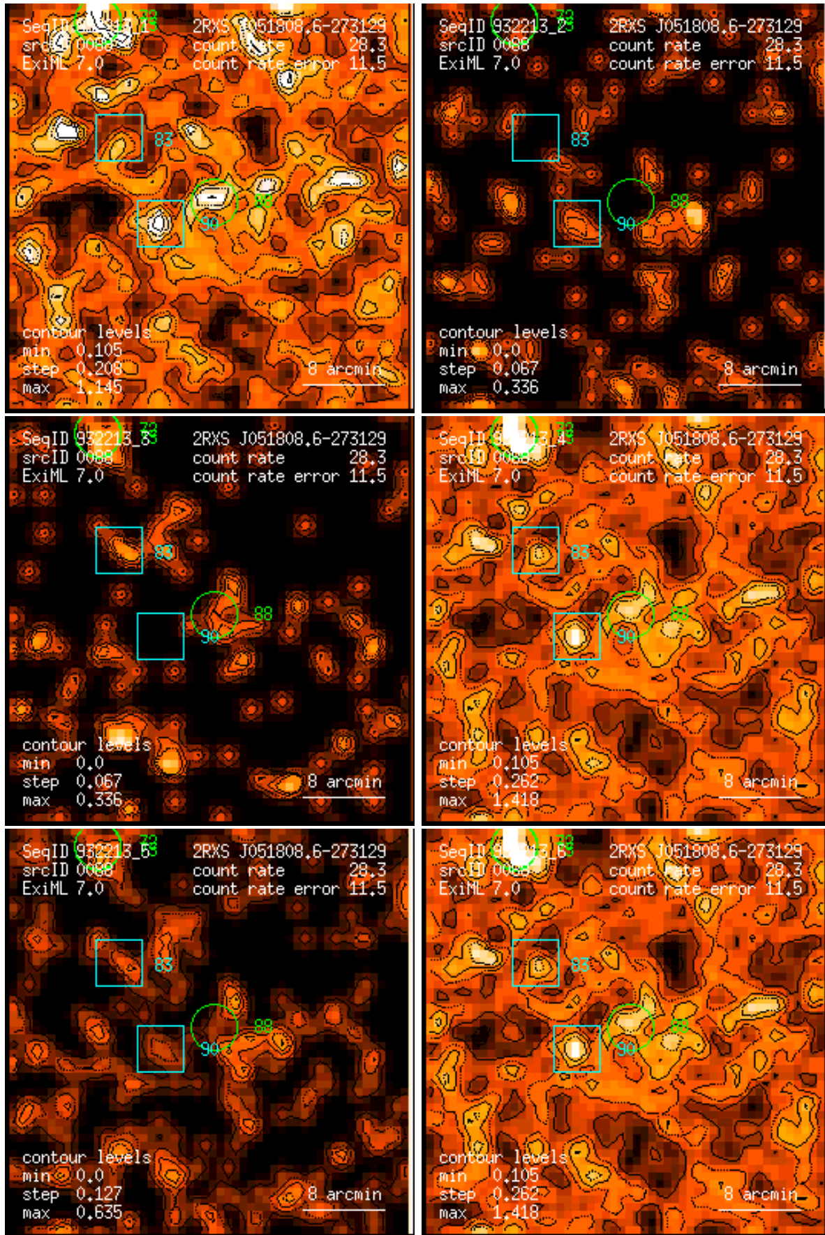
Figure 88: RASS 932213: detection 0088: band rate images, Gaussian filter: (1) PSPC channels 11 – 41, (2) 52 – 90, (3) 91 – 201, (4) 11 – 235, (5) 52 – 201, (6) 11 – 201. Broad band rates in counts/ks. Band rate contour levels in counts/ks/arcmin 2 .
