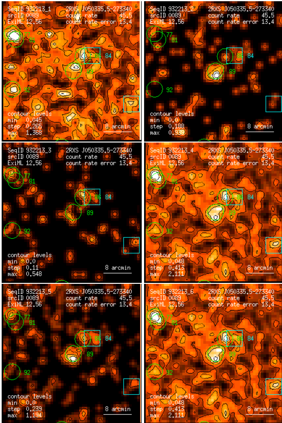
Figure 89: RASS 932213: detection 0089: band rate images, Gaussian filter: (1) PSPC channels 11 – 41, (2) 52 – 90, (3) 91 – 201, (4) 11 – 235, (5) 52 – 201, (6) 11 – 201. Broad band rates in counts/ks. Band rate contour levels in counts/ks/arcmin 2 .
