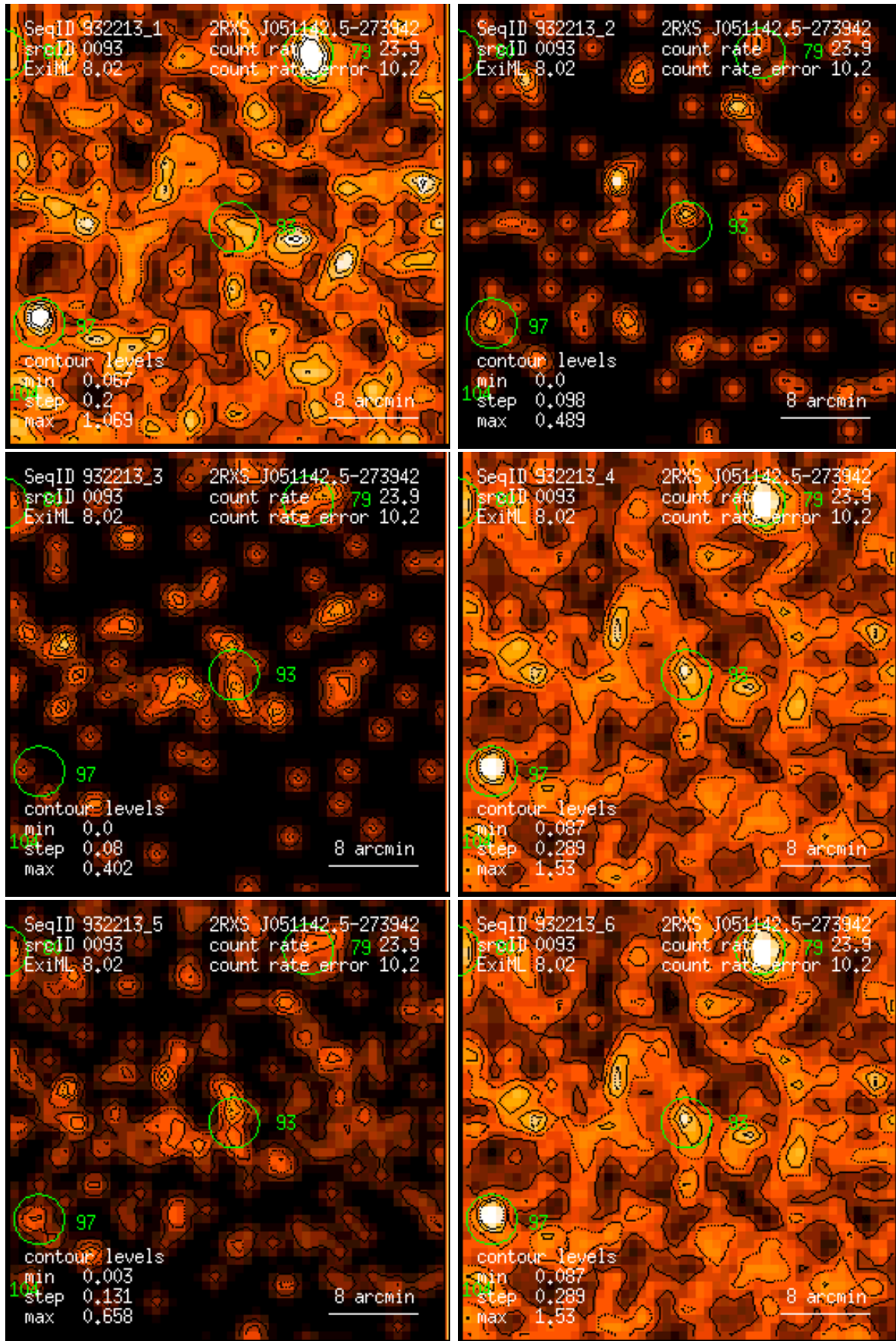
Figure 93: RASS 932213: detection 0093: band rate images, Gaussian filter: (1) PSPC channels 11 – 41, (2) 52 – 90, (3) 91 – 201, (4) 11 – 235, (5) 52 – 201, (6) 11 – 201. Broad band rates in counts/ks. Band rate contour levels in counts/ks/arcmin 2 .
