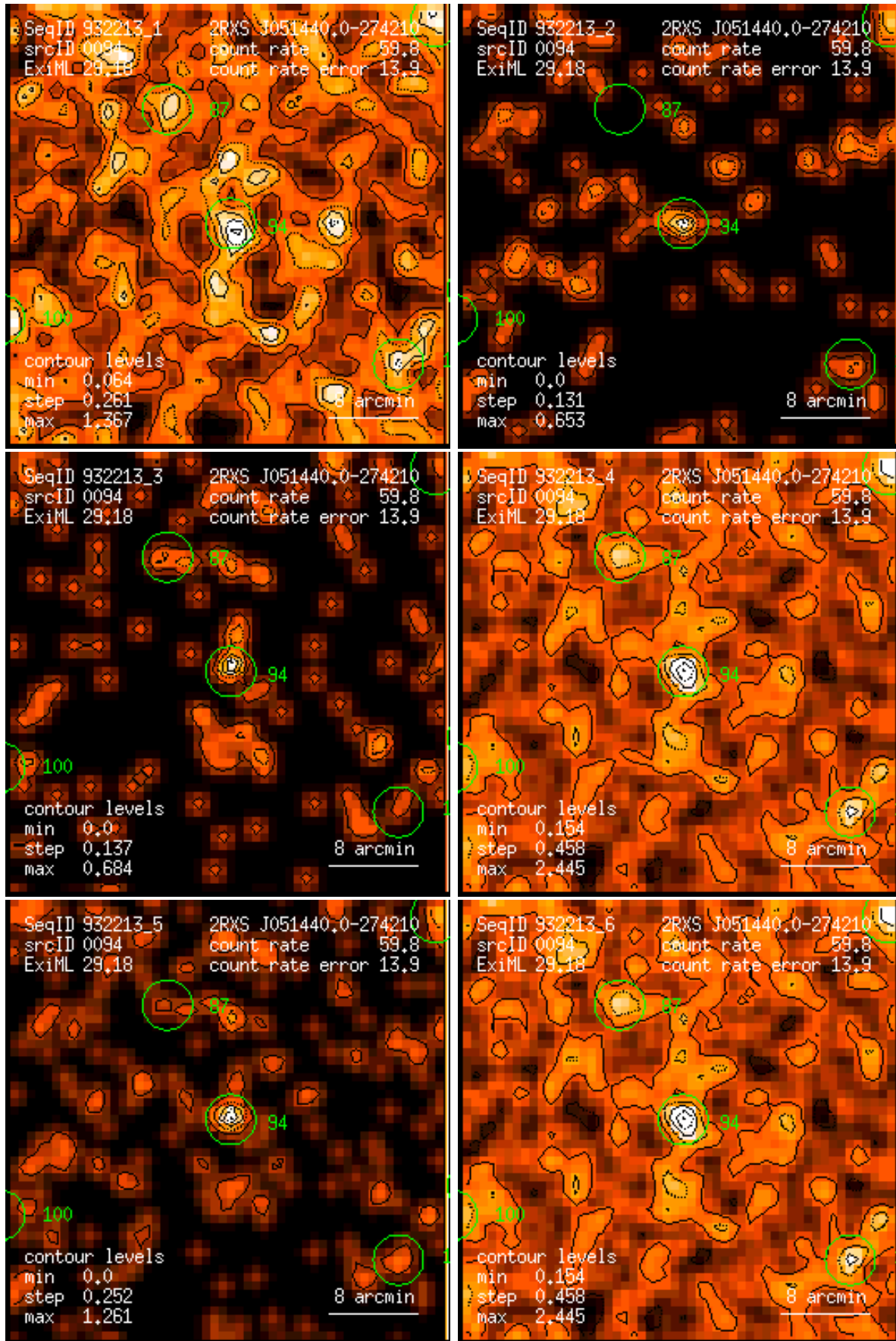
Figure 94: RASS 932213: detection 0094: band rate images, Gaussian filter: (1) PSPC channels 11 – 41, (2) 52 – 90, (3) 91 – 201, (4) 11 – 235, (5) 52 – 201, (6) 11 – 201. Broad band rates in counts/ks. Band rate contour levels in counts/ks/arcmin 2 .
