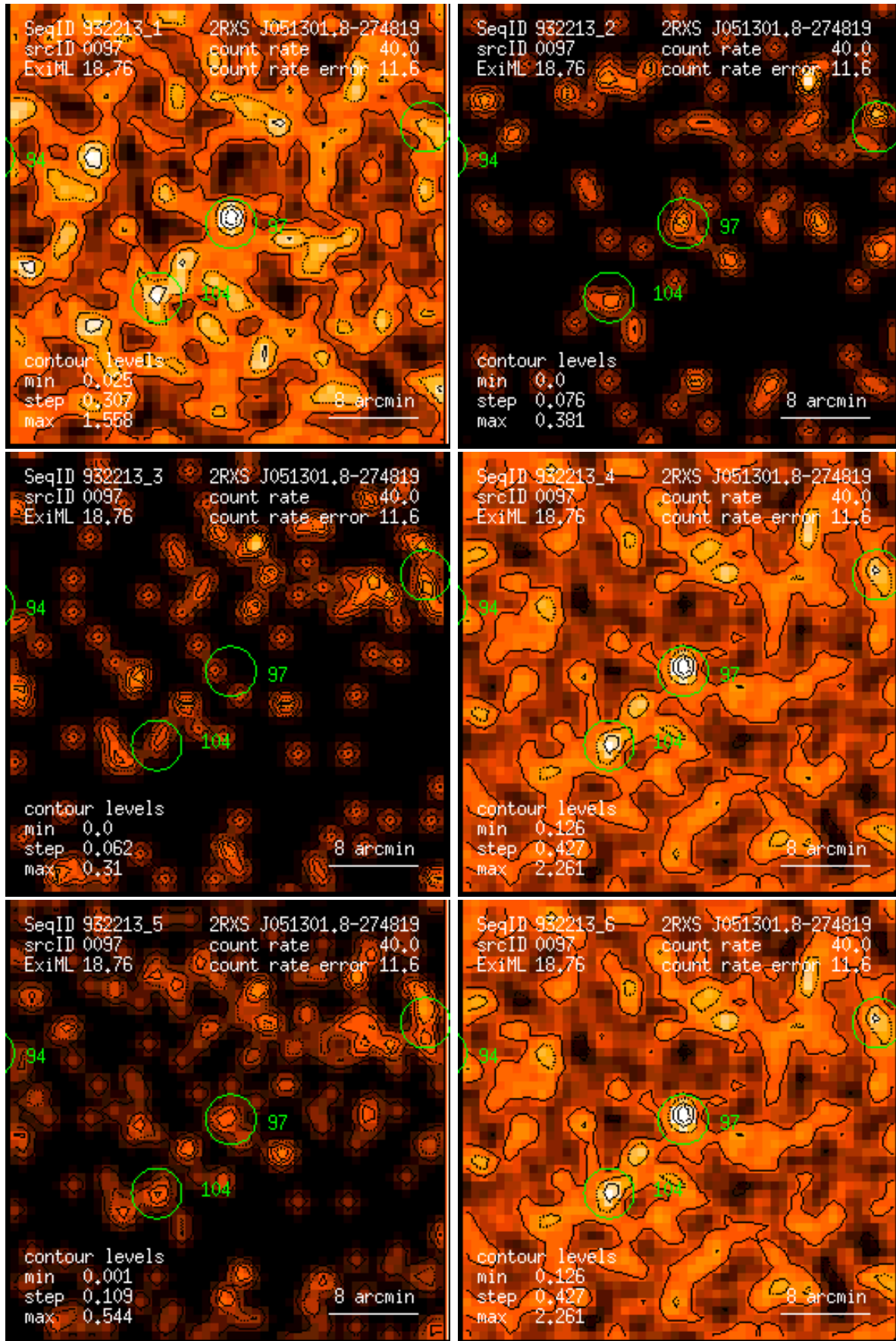
Figure 97: RASS 932213: detection 0097: band rate images, Gaussian filter: (1) PSPC channels 11 – 41, (2) 52 – 90, (3) 91 – 201, (4) 11 – 235, (5) 52 – 201, (6) 11 – 201. Broad band rates in counts/ks. Band rate contour levels in counts/ks/arcmin 2 .
