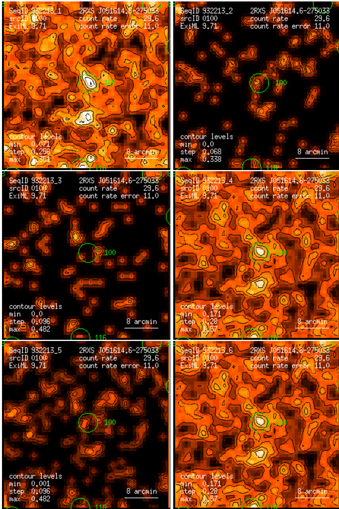
Figure 100: RASS 932213: detection 0100: band rate images, Gaussian filter: (1) PSPC channels 11 – 41, (2) 52 – 90, (3) 91 – 201, (4) 11 – 235, (5) 52 – 201, (6) 11 – 201. Broad band rates in counts/ks. Band rate contour levels in counts/ks/arcmin 2 .
