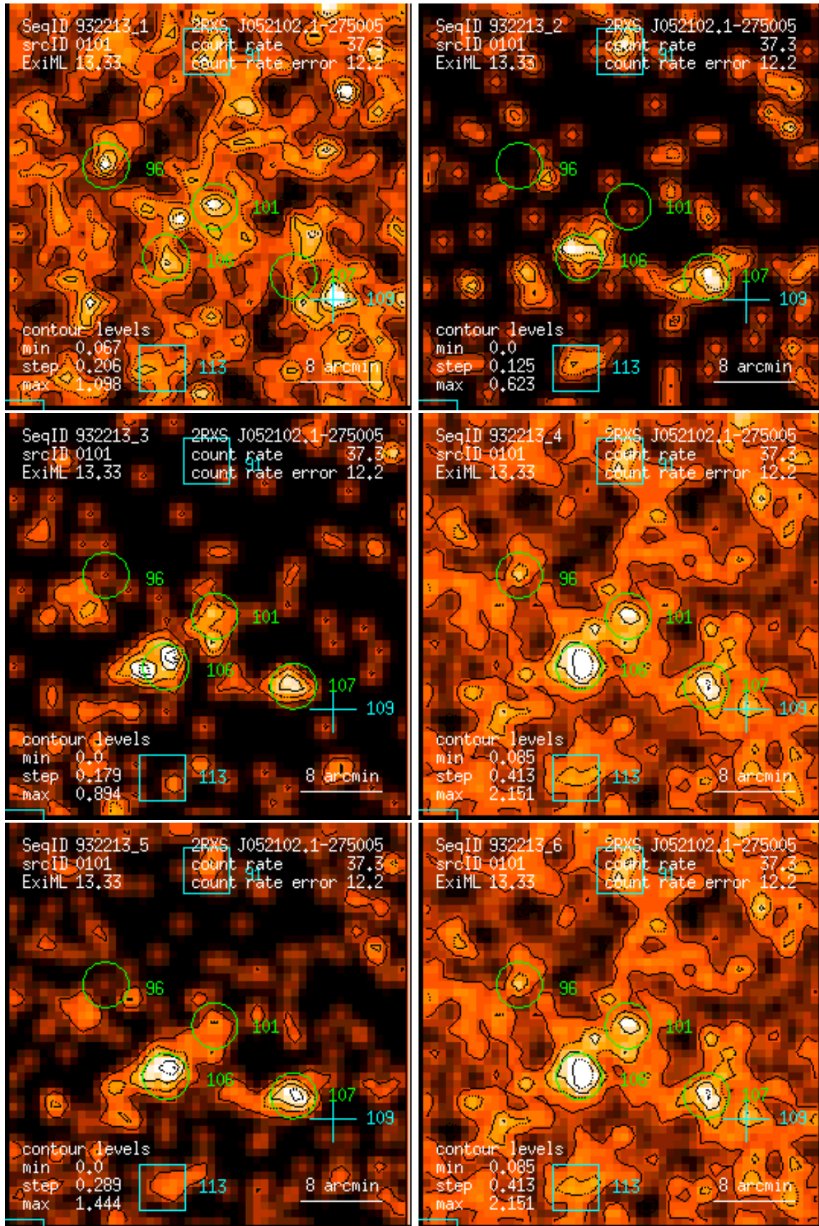
Figure 101: RASS 932213: detection 0101: band rate images, Gaussian filter: (1) PSPC channels 11 – 41, (2) 52 – 90, (3) 91 – 201, (4) 11 – 235, (5) 52 – 201, (6) 11 – 201. Broad band rates in counts/ks. Band rate contour levels in counts/ks/arcmin 2 .
