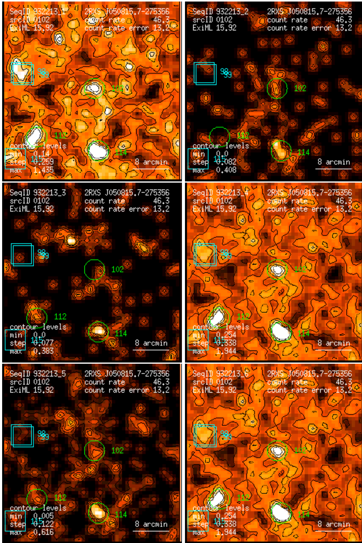
Figure 102: RASS 932213: detection 0102: band rate images, Gaussian filter: (1) PSPC channels 11 – 41, (2) 52 – 90, (3) 91 – 201, (4) 11 – 235, (5) 52 – 201, (6) 11 – 201. Broad band rates in counts/ks. Band rate contour levels in counts/ks/arcmin 2 .
