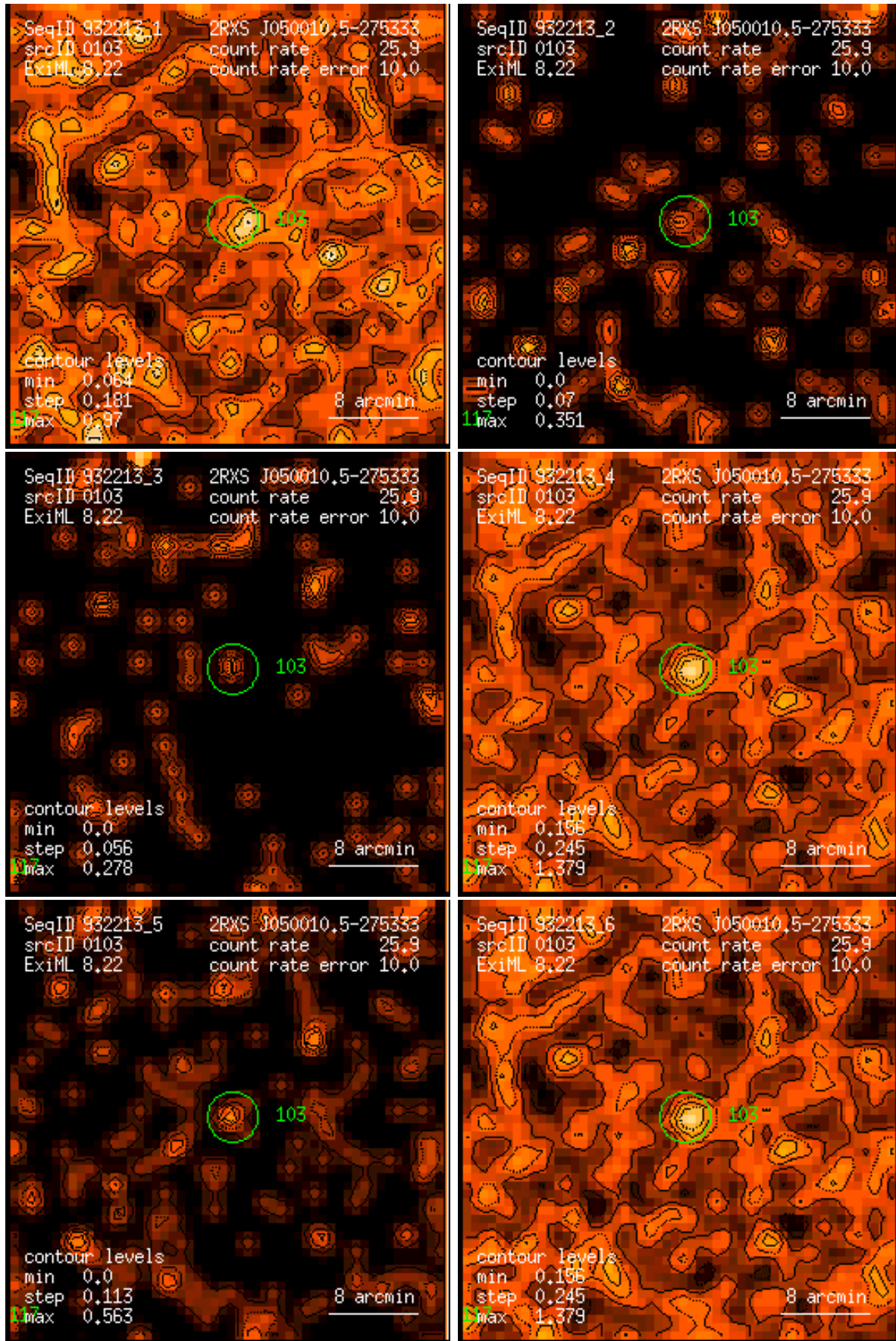
Figure 103: RASS 932213: detection 0103: band rate images, Gaussian filter: (1) PSPC channels 11 – 41, (2) 52 – 90, (3) 91 – 201, (4) 11 – 235, (5) 52 – 201, (6) 11 – 201. Broad band rates in counts/ks. Band rate contour levels in counts/ks/arcmin 2 .
