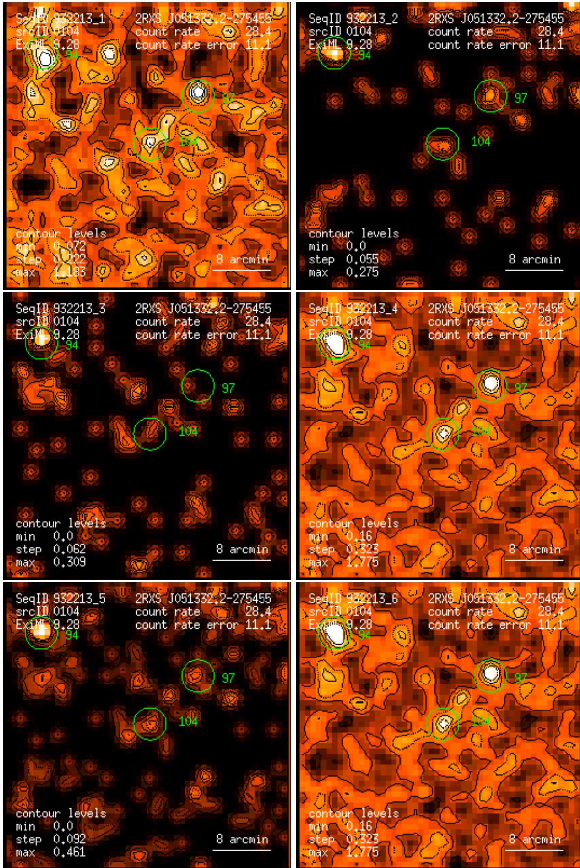
Figure 104: RASS 932213: detection 0104: band rate images, Gaussian filter: (1) PSPC channels 11 – 41, (2) 52 – 90, (3) 91 – 201, (4) 11 – 235, (5) 52 – 201, (6) 11 – 201. Broad band rates in counts/ks. Band rate contour levels in counts/ks/arcmin 2 .
