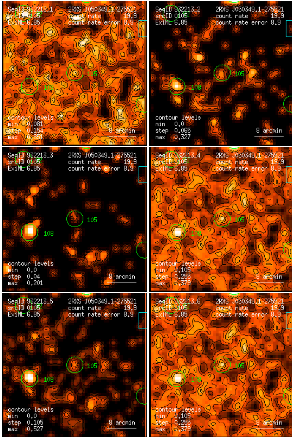
Figure 105: RASS 932213: detection 0105: band rate images, Gaussian filter: (1) PSPC channels 11 – 41, (2) 52 – 90, (3) 91 – 201, (4) 11 – 235, (5) 52 – 201, (6) 11 – 201. Broad band rates in counts/ks. Band rate contour levels in counts/ks/arcmin 2 .
