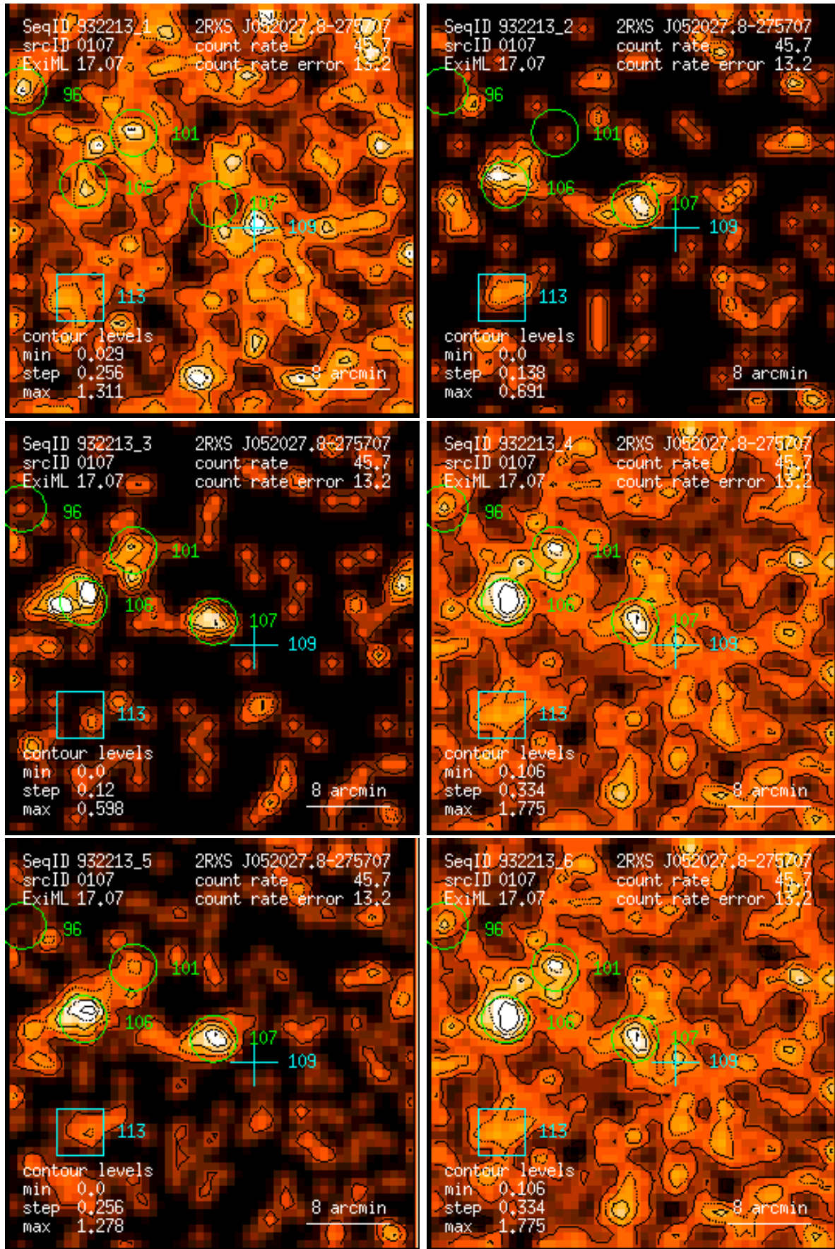
Figure 107: RASS 932213: detection 0107: band rate images, Gaussian filter: (1) PSPC channels 11 – 41, (2) 52 – 90, (3) 91 – 201, (4) 11 – 235, (5) 52 – 201, (6) 11 – 201. Broad band rates in counts/ks. Band rate contour levels in counts/ks/arcmin 2 .
