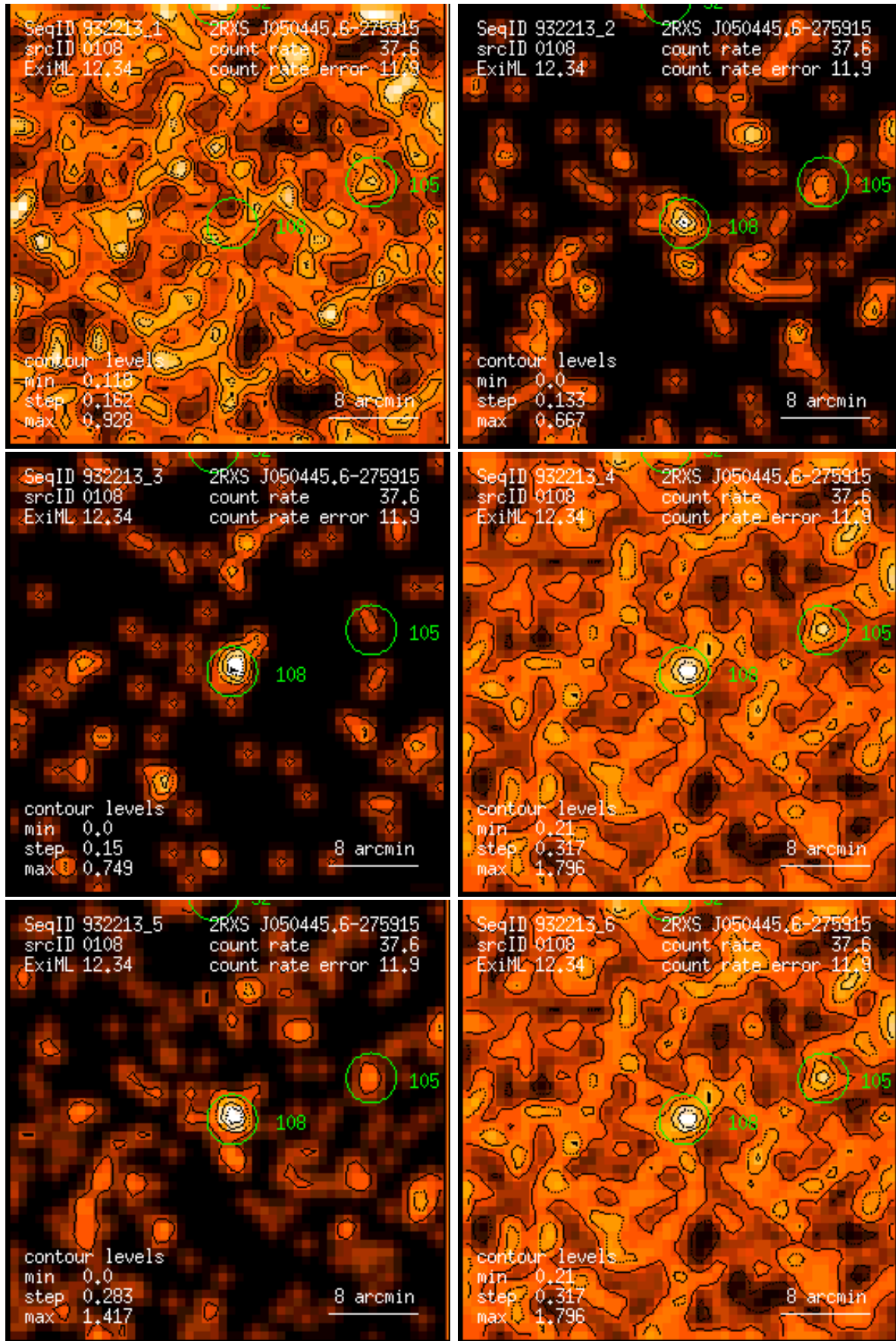
Figure 108: RASS 932213: detection 0108: band rate images, Gaussian filter: (1) PSPC channels 11 – 41, (2) 52 – 90, (3) 91 – 201, (4) 11 – 235, (5) 52 – 201, (6) 11 – 201. Broad band rates in counts/ks. Band rate contour levels in counts/ks/arcmin 2 .
