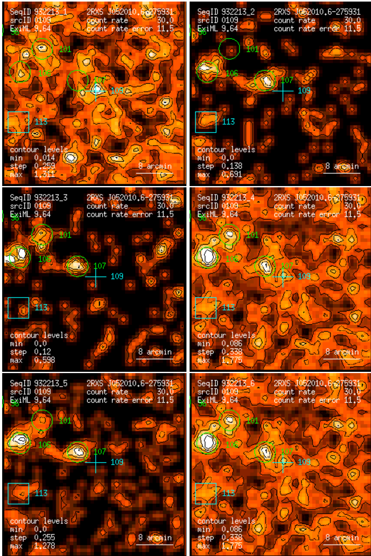
Figure 109: RASS 932213: detection 0109: band rate images, Gaussian filter: (1) PSPC channels 11 – 41, (2) 52 – 90, (3) 91 – 201, (4) 11 – 235, (5) 52 – 201, (6) 11 – 201. Broad band rates in counts/ks. Band rate contour levels in counts/ks/arcmin 2 .
