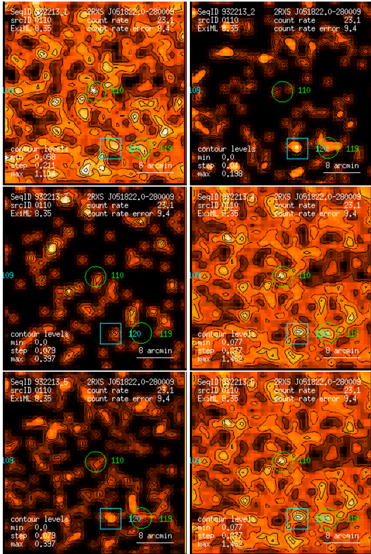
Figure 110: RASS 932213: detection 0110: band rate images, Gaussian filter: (1) PSPC channels 11 – 41, (2) 52 – 90, (3) 91 – 201, (4) 11 – 235, (5) 52 – 201, (6) 11 – 201. Broad band rates in counts/ks. Band rate contour levels in counts/ks/arcmin 2 .
