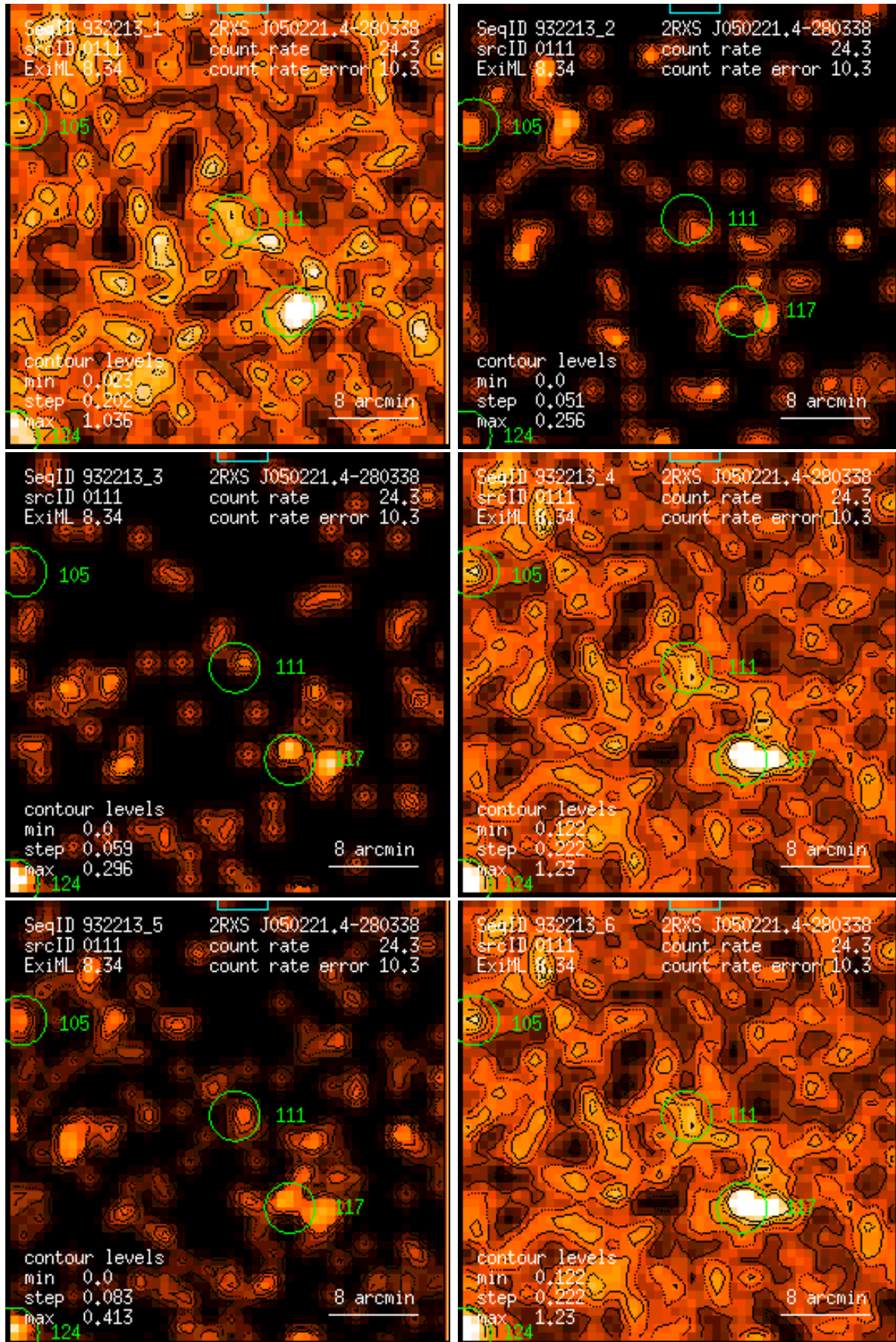
Figure 111: RASS 932213: detection 0111: band rate images, Gaussian filter: (1) PSPC channels 11 – 41, (2) 52 – 90, (3) 91 – 201, (4) 11 – 235, (5) 52 – 201, (6) 11 – 201. Broad band rates in counts/ks. Band rate contour levels in counts/ks/arcmin 2 .
