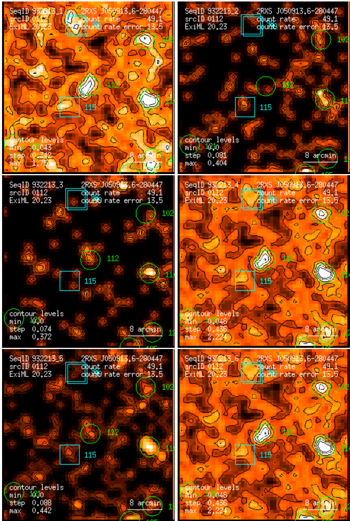
Figure 112: RASS 932213: detection 0112: band rate images, Gaussian filter: (1) PSPC channels 11 – 41, (2) 52 – 90, (3) 91 – 201, (4) 11 – 235, (5) 52 – 201, (6) 11 – 201. Broad band rates in counts/ks. Band rate contour levels in counts/ks/arcmin 2 .
