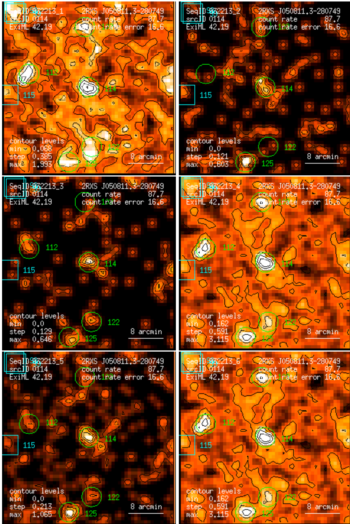
Figure 114: RASS 932213: detection 0114: band rate images, Gaussian filter: (1) PSPC channels 11 – 41, (2) 52 – 90, (3) 91 – 201, (4) 11 – 235, (5) 52 – 201, (6) 11 – 201. Broad band rates in counts/ks. Band rate contour levels in counts/ks/arcmin 2 .
