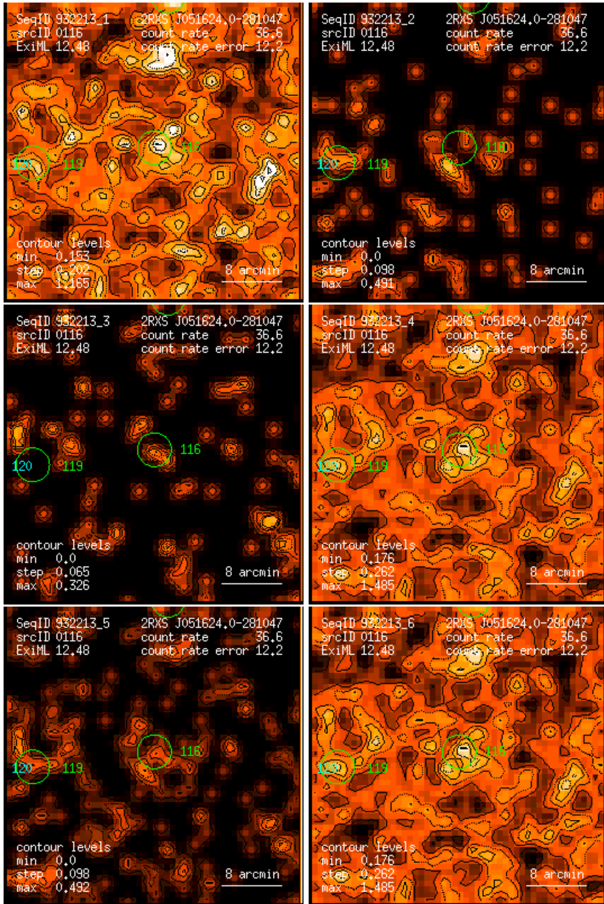
Figure 116: RASS 932213: detection 0116: band rate images, Gaussian filter: (1) PSPC channels 11 – 41, (2) 52 – 90, (3) 91 – 201, (4) 11 – 235, (5) 52 – 201, (6) 11 – 201. Broad band rates in counts/ks. Band rate contour levels in counts/ks/arcmin 2 .
