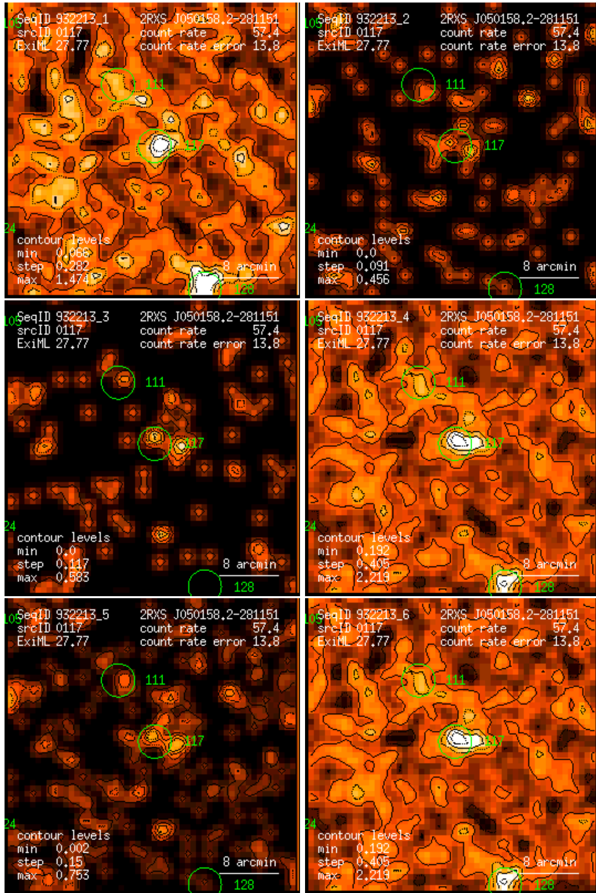
Figure 117: RASS 932213: detection 0117: band rate images, Gaussian filter: (1) PSPC channels 11 – 41, (2) 52 – 90, (3) 91 – 201, (4) 11 – 235, (5) 52 – 201, (6) 11 – 201. Broad band rates in counts/ks. Band rate contour levels in counts/ks/arcmin 2 .
