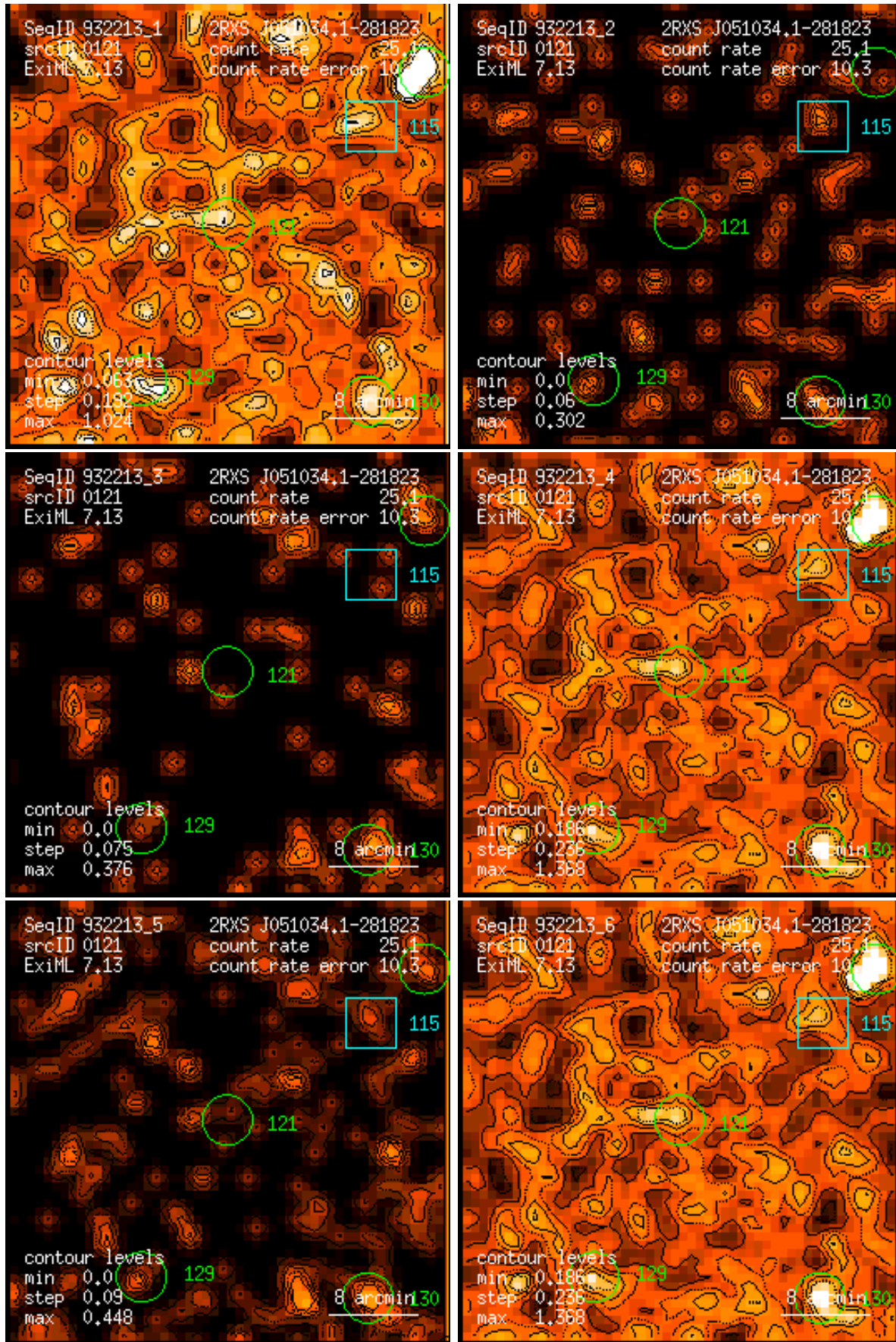
Figure 121: RASS 932213: detection 0121: band rate images, Gaussian filter: (1) PSPC channels 11 – 41, (2) 52 – 90, (3) 91 – 201, (4) 11 – 235, (5) 52 – 201, (6) 11 – 201. Broad band rates in counts/ks. Band rate contour levels in counts/ks/arcmin 2 .
