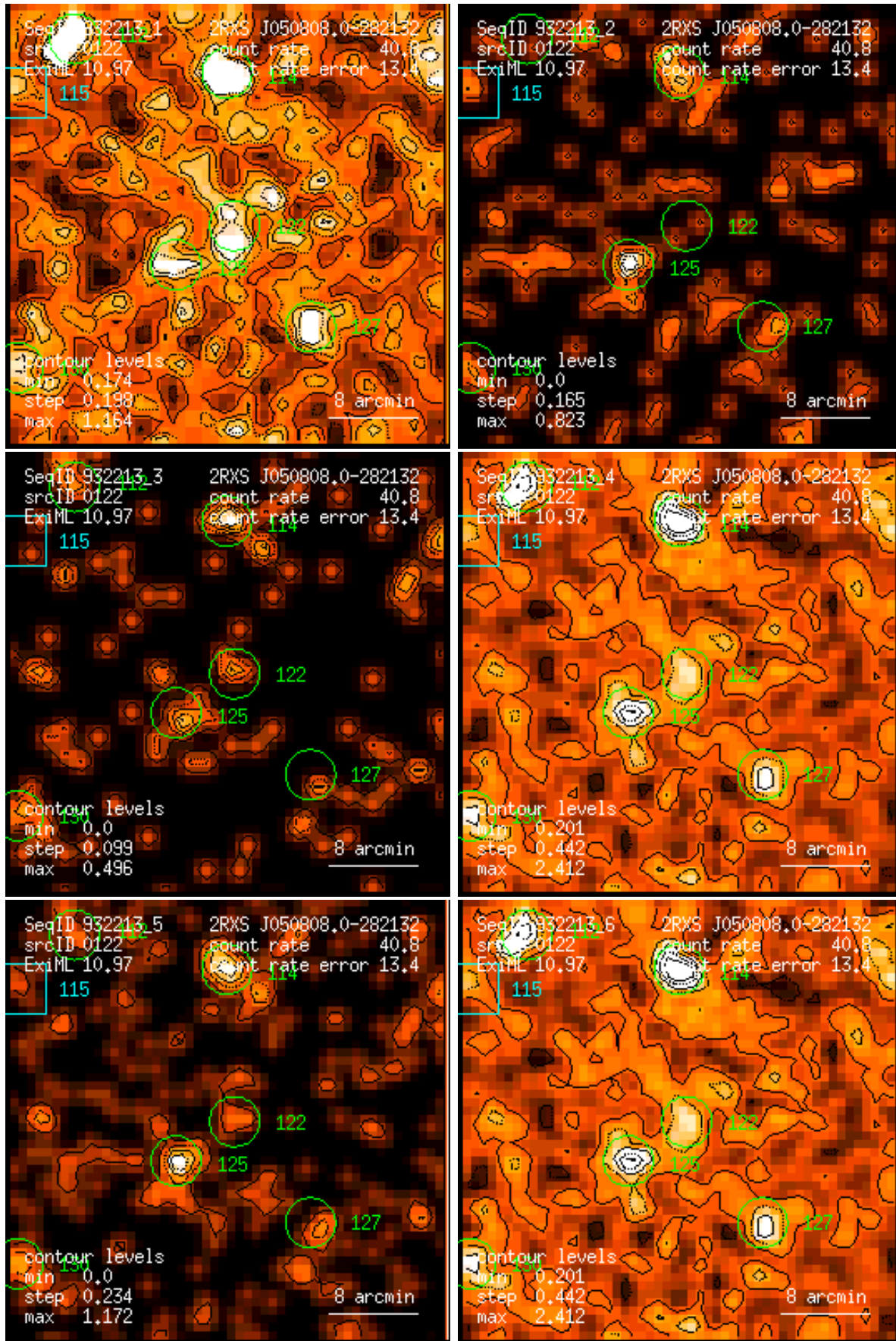
Figure 122: RASS 932213: detection 0122: band rate images, Gaussian filter: (1) PSPC channels 11 – 41, (2) 52 – 90, (3) 91 – 201, (4) 11 – 235, (5) 52 – 201, (6) 11 – 201. Broad band rates in counts/ks. Band rate contour levels in counts/ks/arcmin 2 .
