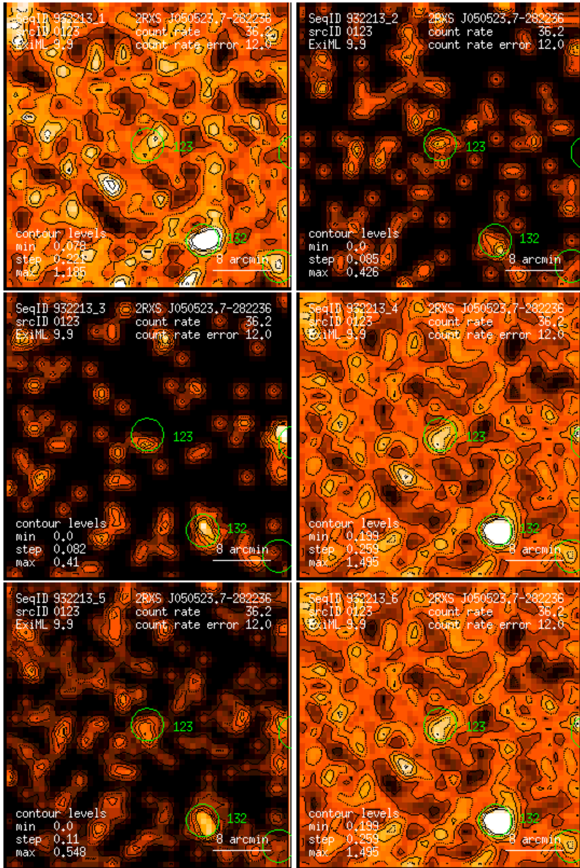
Figure 123: RASS 932213: detection 0123: band rate images, Gaussian filter: (1) PSPC channels 11 – 41, (2) 52 – 90, (3) 91 – 201, (4) 11 – 235, (5) 52 – 201, (6) 11 – 201. Broad band rates in counts/ks. Band rate contour levels in counts/ks/arcmin 2 .
