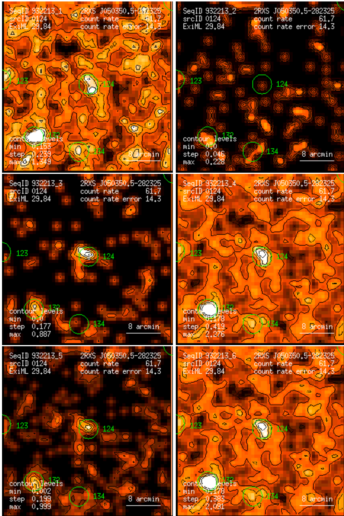
Figure 124: RASS 932213: detection 0124: band rate images, Gaussian filter: (1) PSPC channels 11 – 41, (2) 52 – 90, (3) 91 – 201, (4) 11 – 235, (5) 52 – 201, (6) 11 – 201. Broad band rates in counts/ks. Band rate contour levels in counts/ks/arcmin 2 .
