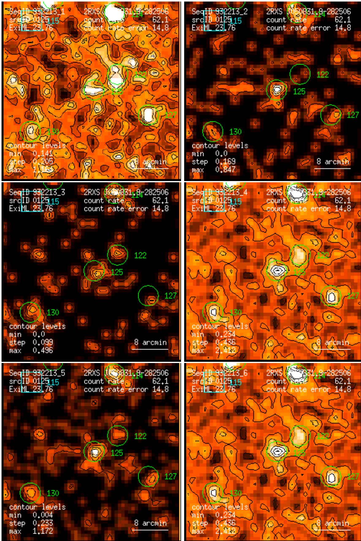
Figure 125: RASS 932213: detection 0125: band rate images, Gaussian filter: (1) PSPC channels 11 – 41, (2) 52 – 90, (3) 91 – 201, (4) 11 – 235, (5) 52 – 201, (6) 11 – 201. Broad band rates in counts/ks. Band rate contour levels in counts/ks/arcmin 2 .
