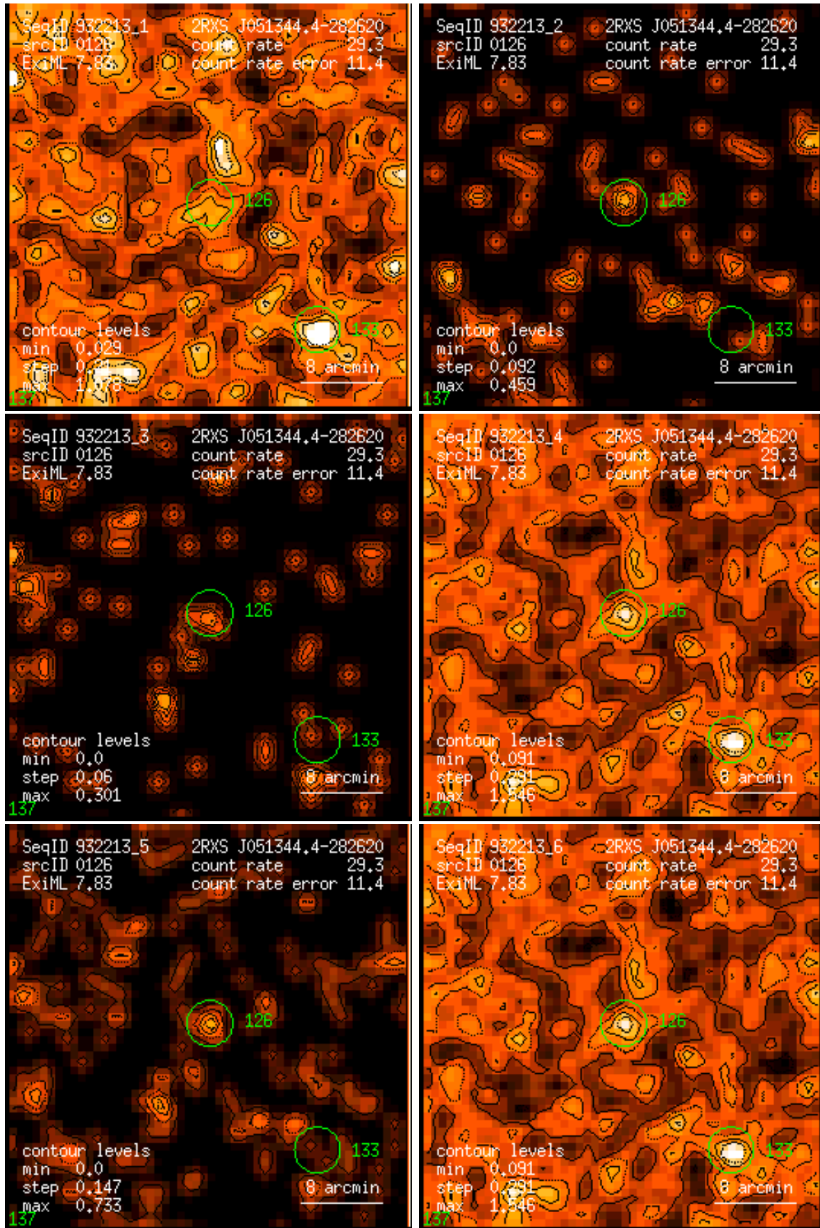
Figure 126: RASS 932213: detection 0126: band rate images, Gaussian filter: (1) PSPC channels 11 – 41, (2) 52 – 90, (3) 91 – 201, (4) 11 – 235, (5) 52 – 201, (6) 11 – 201. Broad band rates in counts/ks. Band rate contour levels in counts/ks/arcmin 2 .
