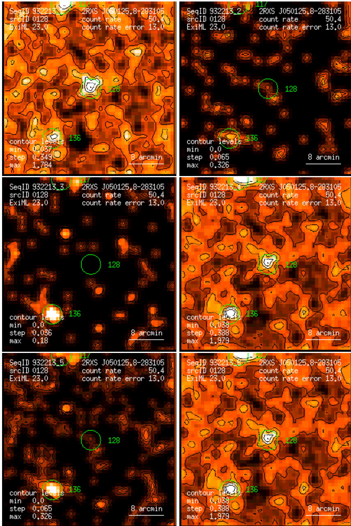
Figure 128: RASS 932213: detection 0128: band rate images, Gaussian filter: (1) PSPC channels 11 – 41, (2) 52 – 90, (3) 91 – 201, (4) 11 – 235, (5) 52 – 201, (6) 11 – 201. Broad band rates in counts/ks. Band rate contour levels in counts/ks/arcmin 2 .
