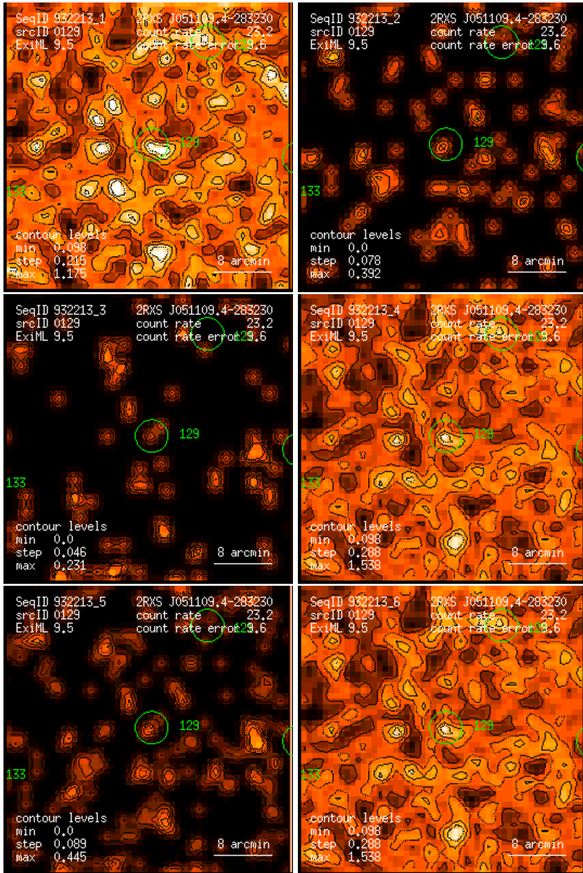
Figure 129: RASS 932213: detection 0129: band rate images, Gaussian filter: (1) PSPC channels 11 – 41, (2) 52 – 90, (3) 91 – 201, (4) 11 – 235, (5) 52 – 201, (6) 11 – 201. Broad band rates in counts/ks. Band rate contour levels in counts/ks/arcmin 2 .
