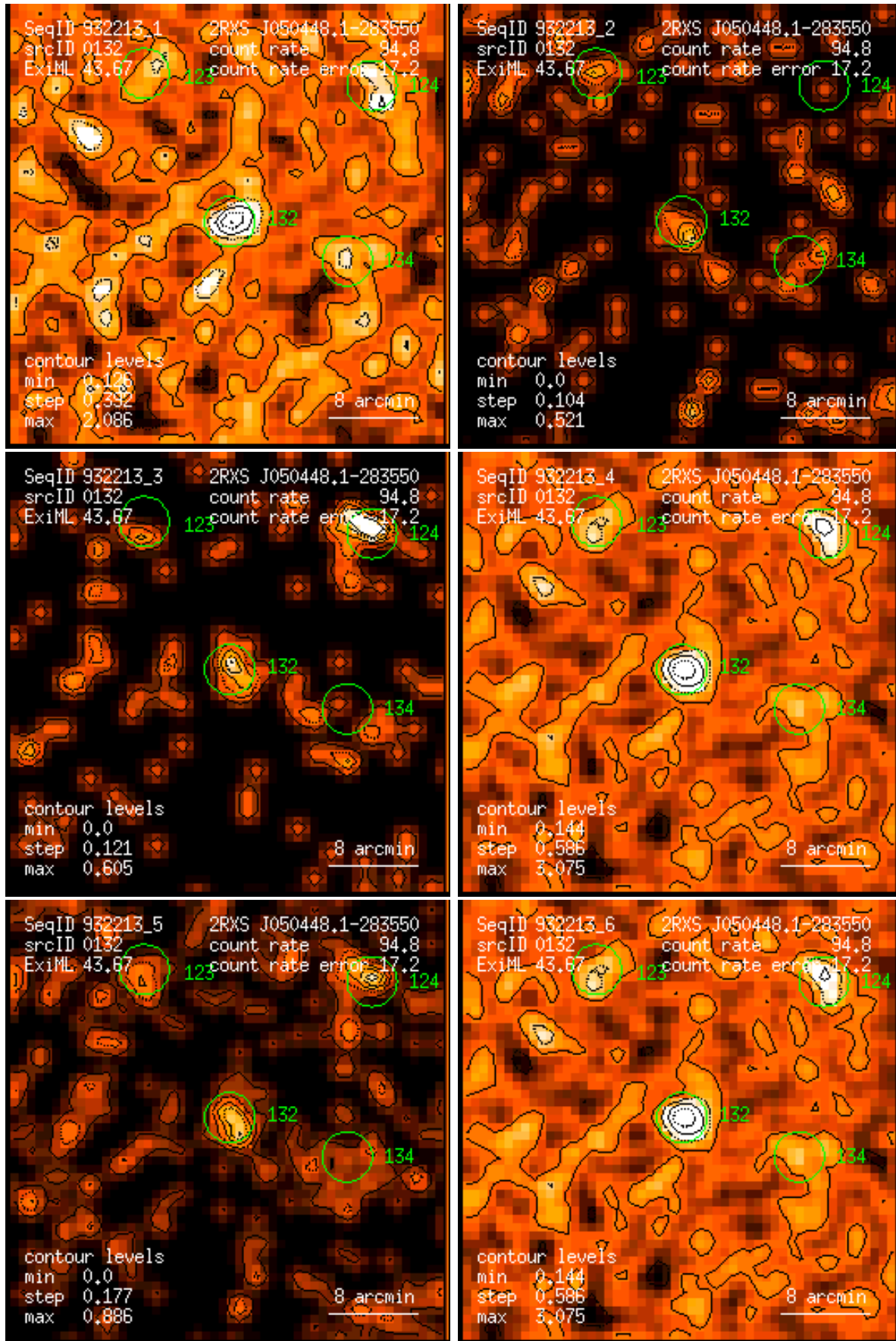
Figure 132: RASS 932213: detection 0132: band rate images, Gaussian filter: (1) PSPC channels 11 – 41, (2) 52 – 90, (3) 91 – 201, (4) 11 – 235, (5) 52 – 201, (6) 11 – 201. Broad band rates in counts/ks. Band rate contour levels in counts/ks/arcmin 2 .
