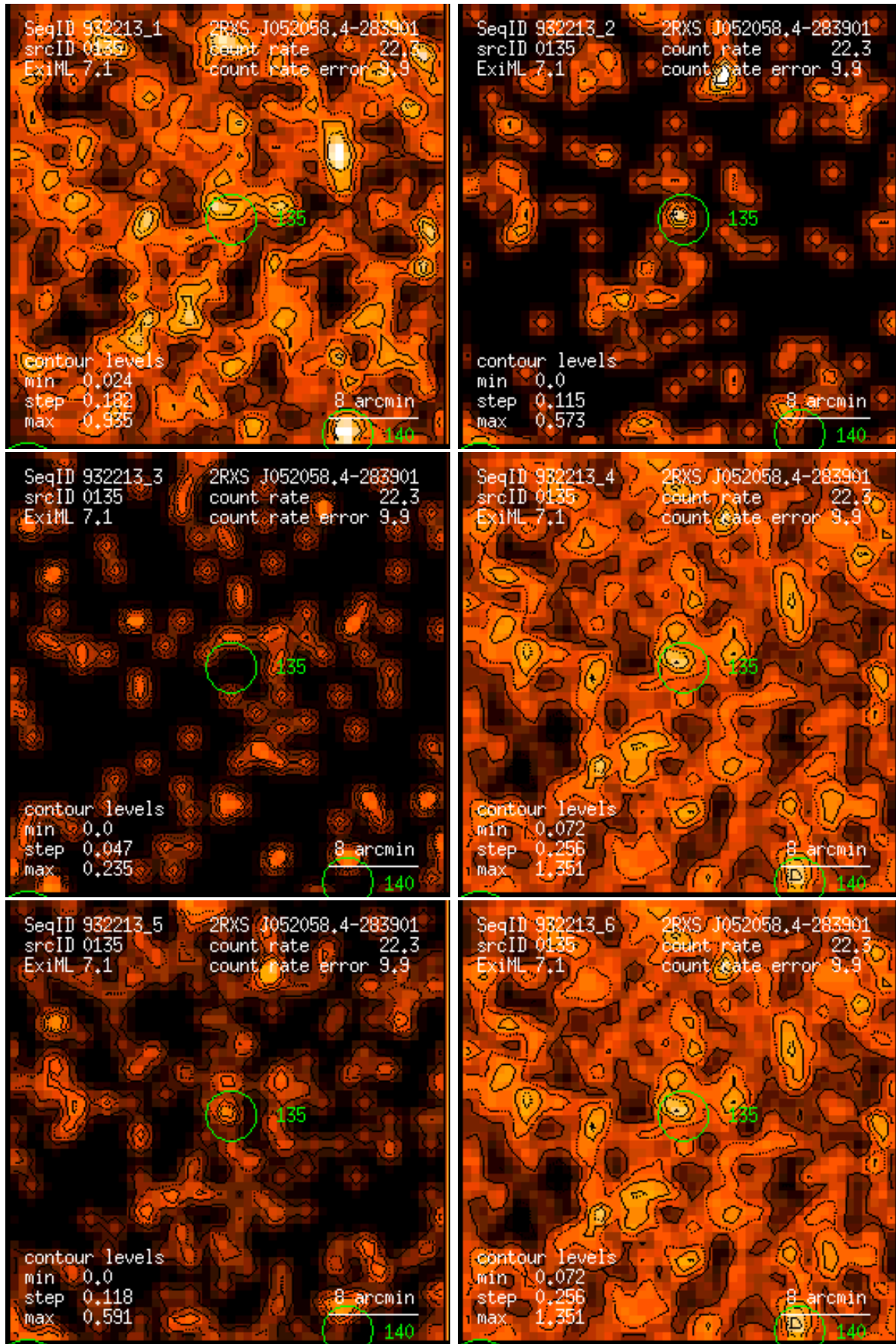
Figure 135: RASS 932213: detection 0135: band rate images, Gaussian filter: (1) PSPC channels 11 – 41, (2) 52 – 90, (3) 91 – 201, (4) 11 – 235, (5) 52 – 201, (6) 11 – 201. Broad band rates in counts/ks. Band rate contour levels in counts/ks/arcmin 2 .
