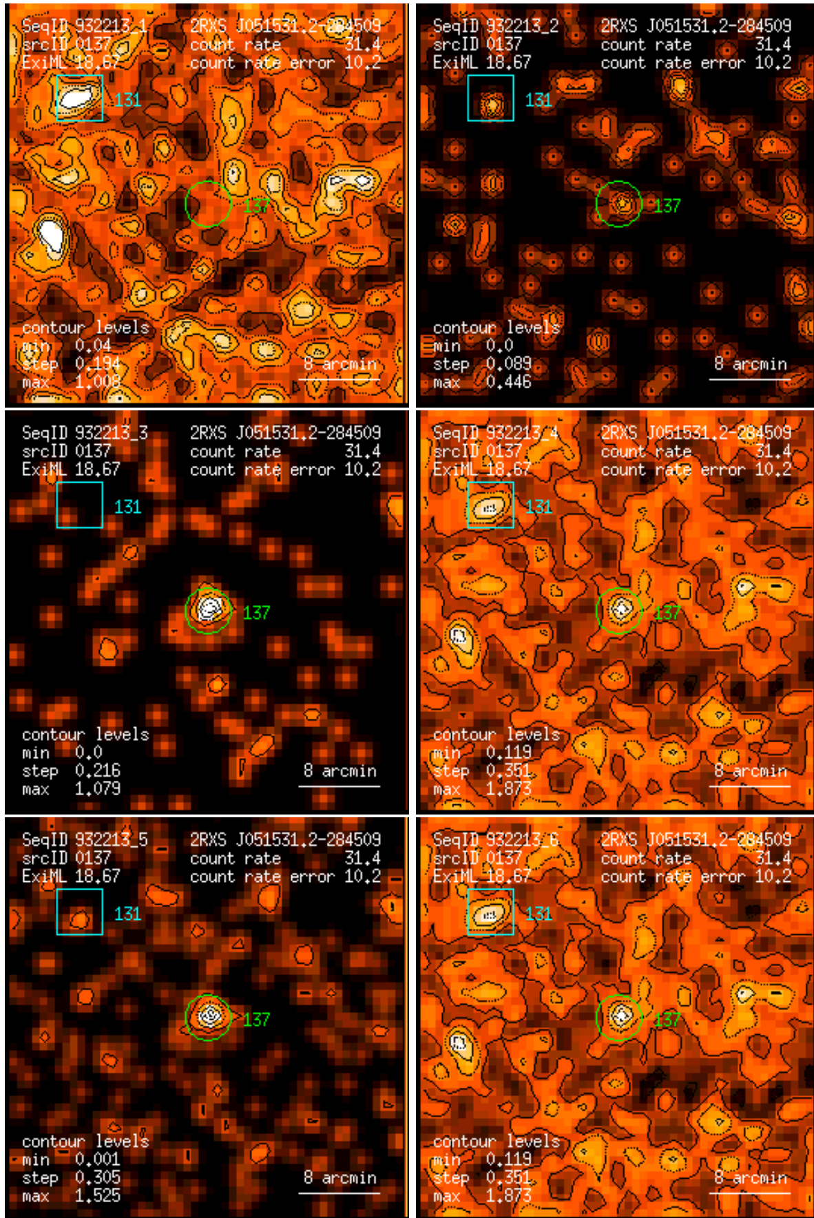
Figure 137: RASS 932213: detection 0137: band rate images, Gaussian filter: (1) PSPC channels 11 – 41, (2) 52 – 90, (3) 91 – 201, (4) 11 – 235, (5) 52 – 201, (6) 11 – 201. Broad band rates in counts/ks. Band rate contour levels in counts/ks/arcmin 2 .
