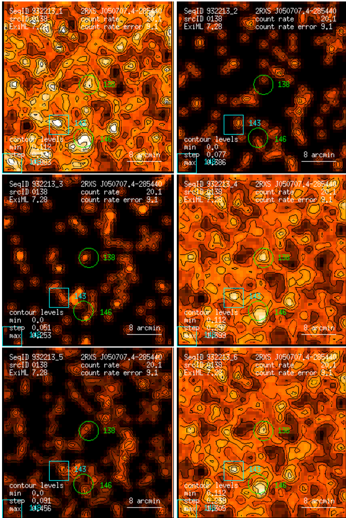
Figure 138: RASS 932213: detection 0138: band rate images, Gaussian filter: (1) PSPC channels 11 – 41, (2) 52 – 90, (3) 91 – 201, (4) 11 – 235, (5) 52 – 201, (6) 11 – 201. Broad band rates in counts/ks. Band rate contour levels in counts/ks/arcmin 2 .
