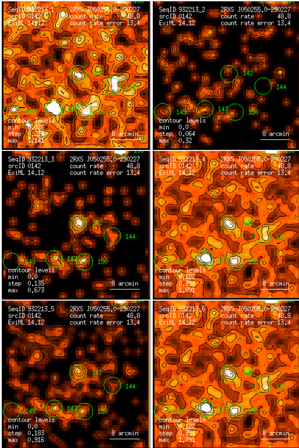
Figure 142: RASS 932213: detection 0142: band rate images, Gaussian filter: (1) PSPC channels 11 – 41, (2) 52 – 90, (3) 91 – 201, (4) 11 – 235, (5) 52 – 201, (6) 11 – 201. Broad band rates in counts/ks. Band rate contour levels in counts/ks/arcmin 2 .
