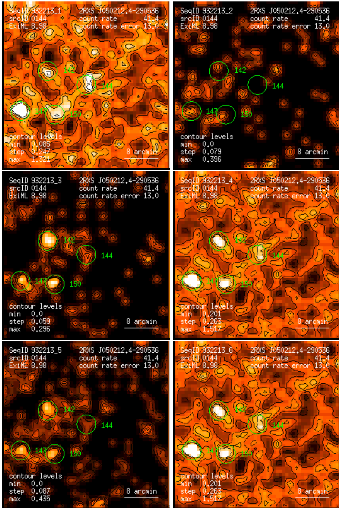
Figure 144: RASS 932213: detection 0144: band rate images, Gaussian filter: (1) PSPC channels 11 – 41, (2) 52 – 90, (3) 91 – 201, (4) 11 – 235, (5) 52 – 201, (6) 11 – 201. Broad band rates in counts/ks. Band rate contour levels in counts/ks/arcmin 2 .
