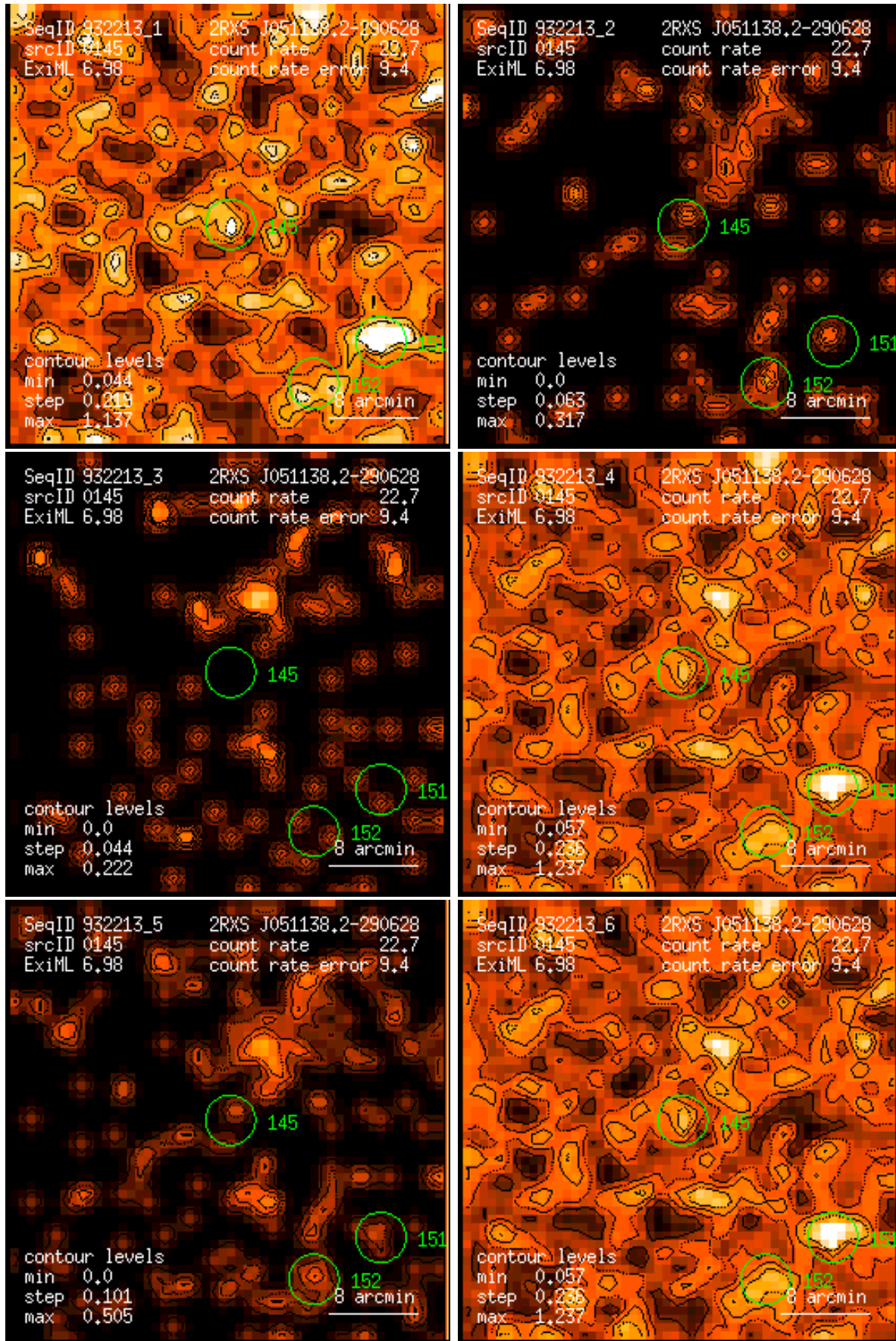
Figure 145: RASS 932213: detection 0145: band rate images, Gaussian filter: (1) PSPC channels 11 – 41, (2) 52 – 90, (3) 91 – 201, (4) 11 – 235, (5) 52 – 201, (6) 11 – 201. Broad band rates in counts/ks. Band rate contour levels in counts/ks/arcmin 2 .
