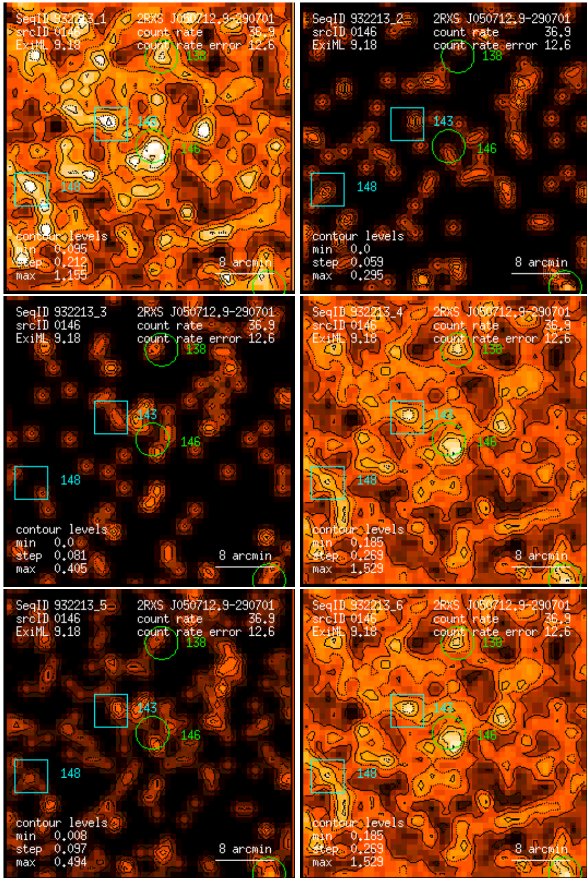
Figure 146: RASS 932213: detection 0146: band rate images, Gaussian filter: (1) PSPC channels 11 – 41, (2) 52 – 90, (3) 91 – 201, (4) 11 – 235, (5) 52 – 201, (6) 11 – 201. Broad band rates in counts/ks. Band rate contour levels in counts/ks/arcmin 2 .
