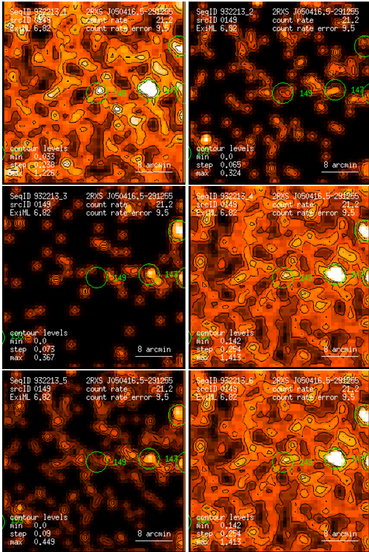
Figure 149: RASS 932213: detection 0149: band rate images, Gaussian filter: (1) PSPC channels 11 – 41, (2) 52 – 90, (3) 91 – 201, (4) 11 – 235, (5) 52 – 201, (6) 11 – 201. Broad band rates in counts/ks. Band rate contour levels in counts/ks/arcmin 2 .
