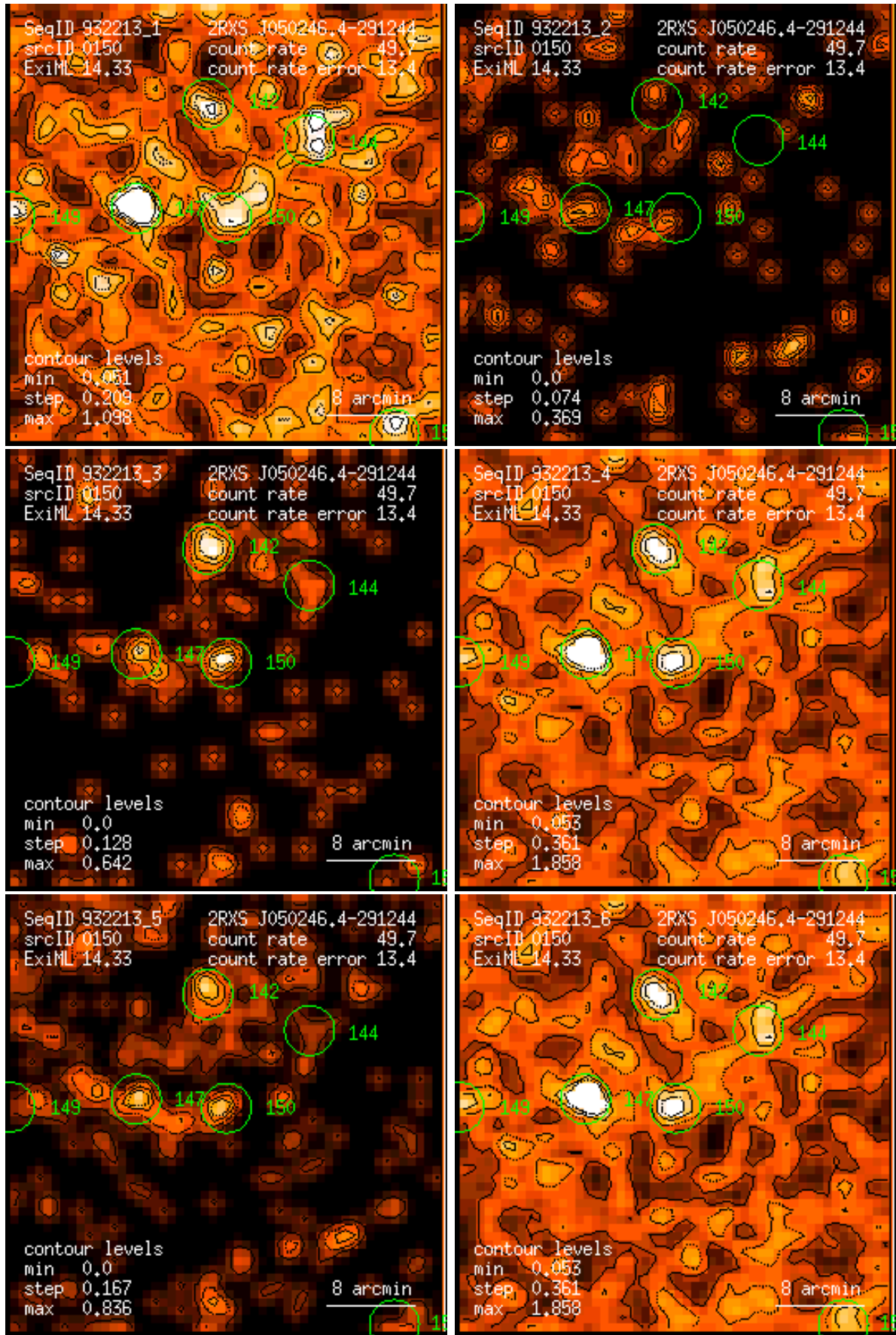
Figure 150: RASS 932213: detection 0150: band rate images, Gaussian filter: (1) PSPC channels 11 – 41, (2) 52 – 90, (3) 91 – 201, (4) 11 – 235, (5) 52 – 201, (6) 11 – 201. Broad band rates in counts/ks. Band rate contour levels in counts/ks/arcmin 2 .
