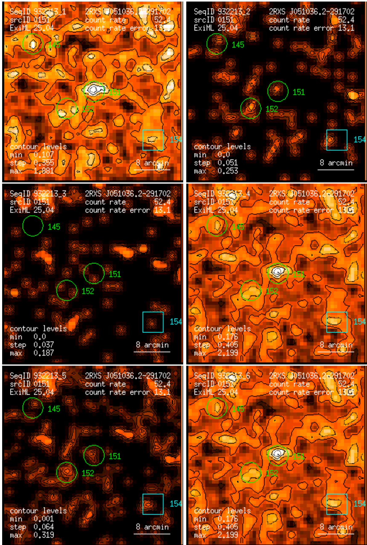
Figure 151: RASS 932213: detection 0151: band rate images, Gaussian filter: (1) PSPC channels 11 – 41, (2) 52 – 90, (3) 91 – 201, (4) 11 – 235, (5) 52 – 201, (6) 11 – 201. Broad band rates in counts/ks. Band rate contour levels in counts/ks/arcmin 2 .
